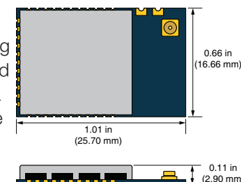
Figure 1: Package Dimensions
