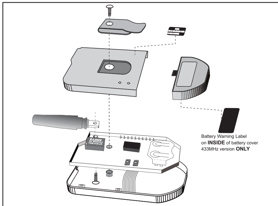
Figure 5: OTX-***-HH-LR8-MS Assembly
