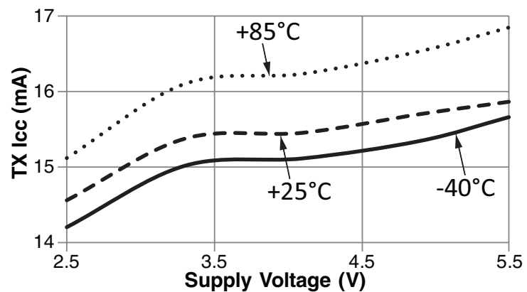
Figure 10: TT Series Transceiver TX Current Consumption vs. Supply Voltage at 0dBm
