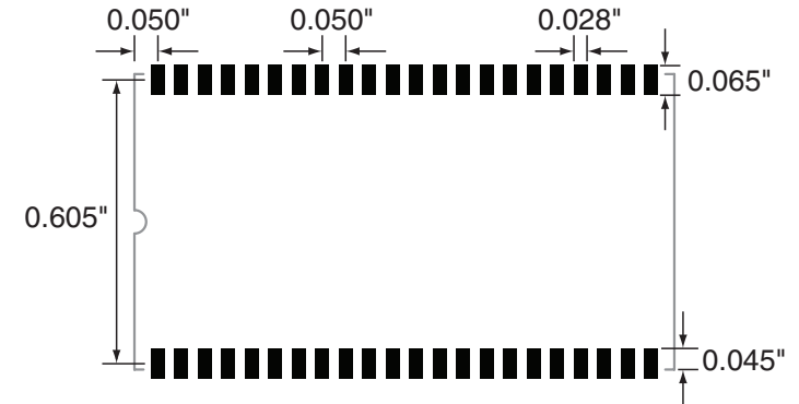
Figure 27: Recommended PCB Layout
