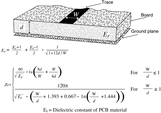
Figure 28: Microstrip Formulas
