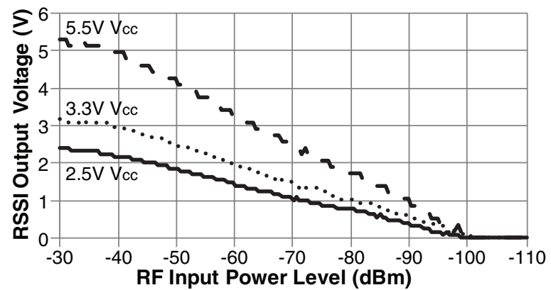
Figure 12: TT Series Transceiver RSSI Voltage vs. Input Power
