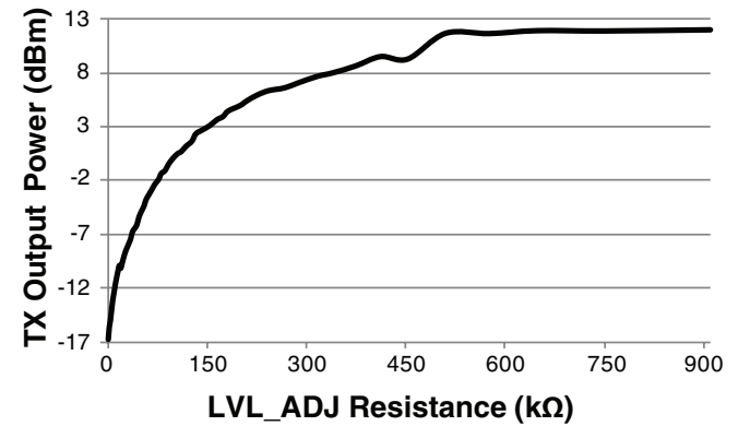
Figure 6: TT Series Transceiver Output Power vs. LVL_ADJ Resistance
