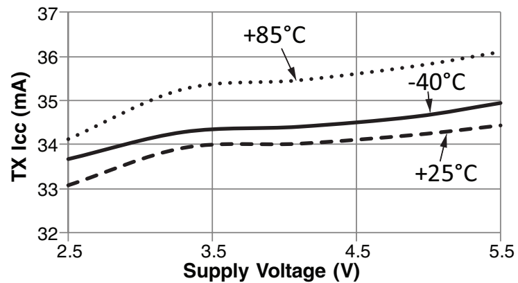
Figure 9: TT Series Transceiver TX Current Consumption vs. Supply Voltage at +12.5dBm
