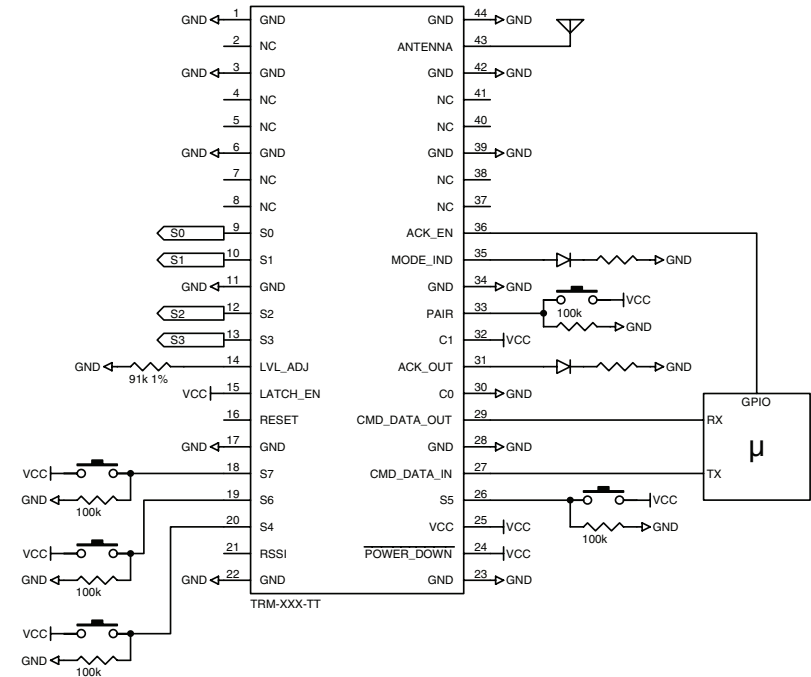
Figure 23: TT Series Transceiver Typical Application Circuit with External Microprocessor
