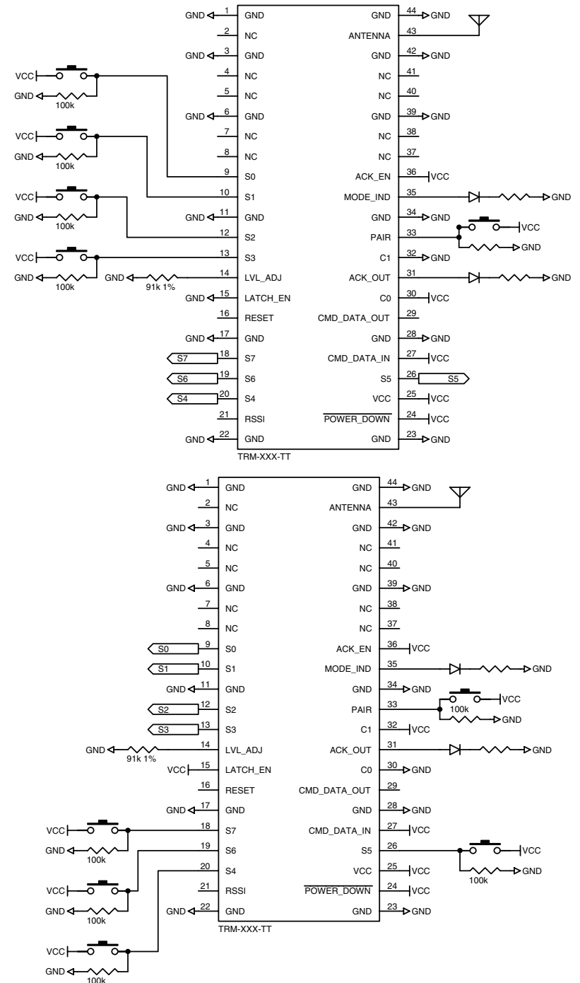
Figure 16: TT Series Transceiver Basic Application Circuits for Bi-directional Remote Control
