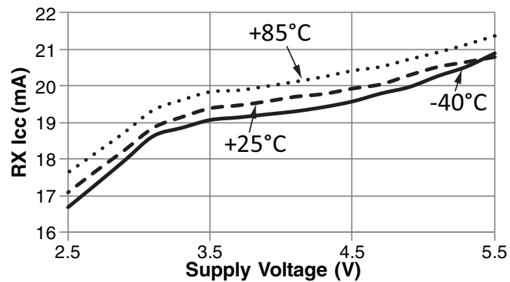
Figure 11: TT Series Transceiver RX Current Consumption vs. Supply Voltage
