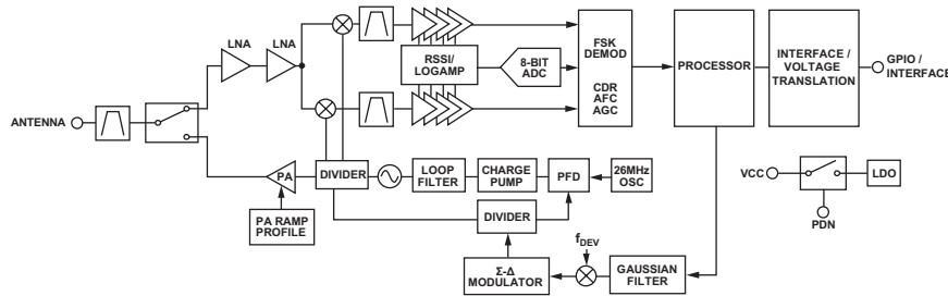
Figure 15: TT Series Transceiver RF Section Block Diagram
