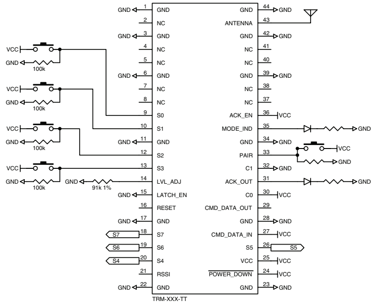
Figure 22: TT Series Transceiver Basic Application Circuit
