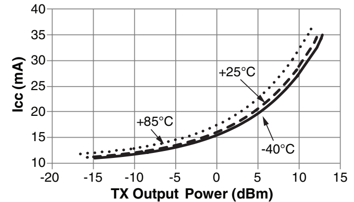
Figure 8: TT Series Transceiver Current Consumption vs. Transmitter Output Power at 5.5V
