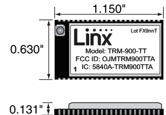
Figure 1: Package Dimensions
