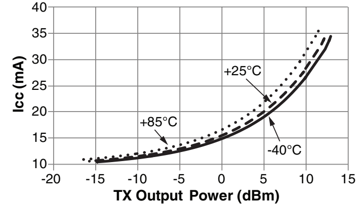
Figure 7: TT Series Transceiver Current Consumption vs. Transmitter Output Power at 3.3V
