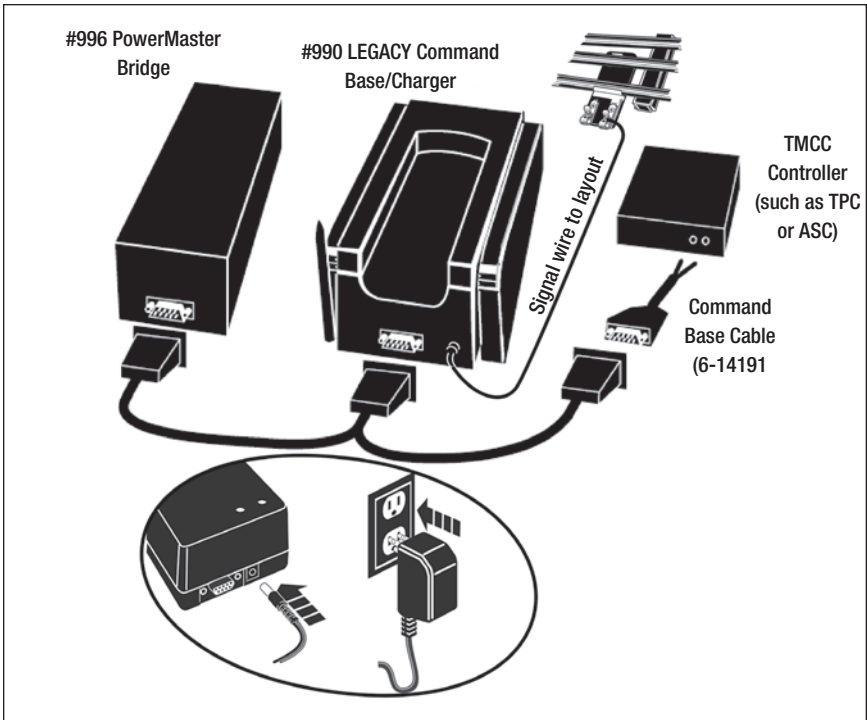
Figure 1. Connecting your PowerMaster Bridge
