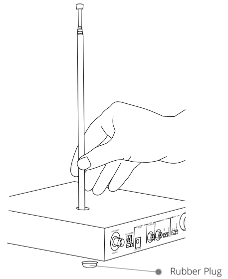
LT-800/LT-803 shown with top mount antenna connected through top of unit (part numbers LA-101, LA-106 (72 MHz) or LA-102 (216 MHz))
