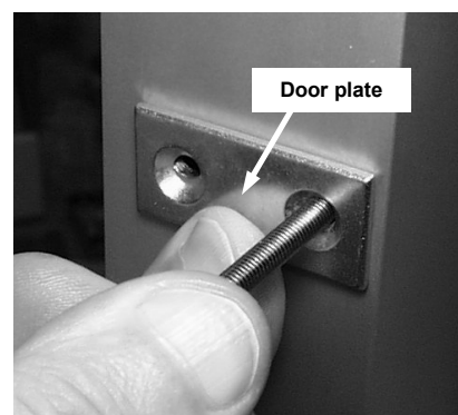
Fig. 9: Secure lock to door -- loosely at first
