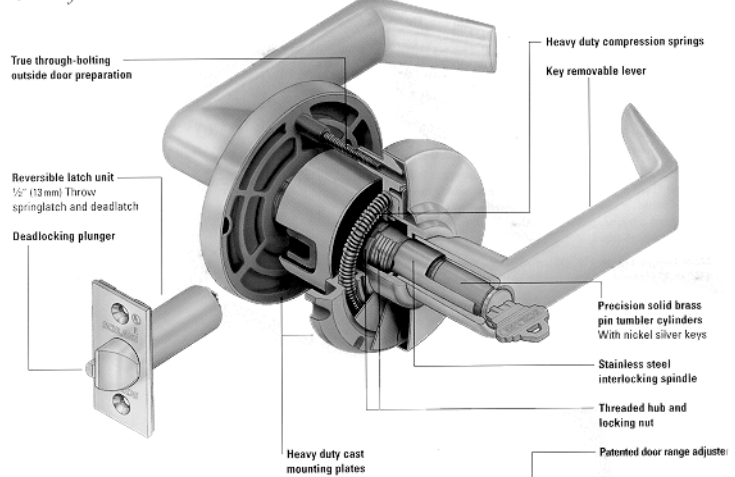
Cutaway View
