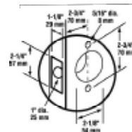
Door Preparation
