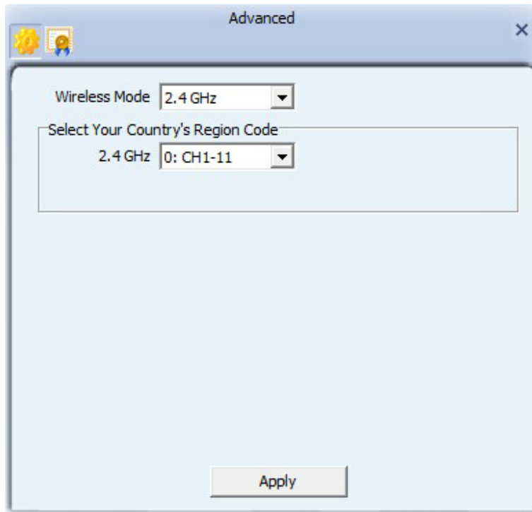
Figure 2-1-6 Advance page
