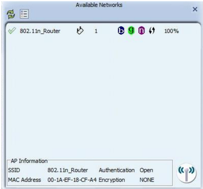
Figure 2-1-5 Network page
