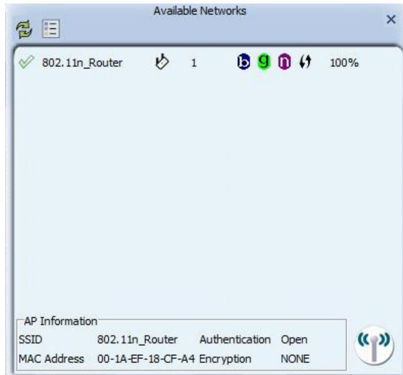
Figure 2-3-1-1 Network function
