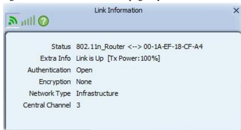
Figure 2-5-1 Statistics function
