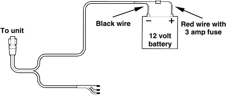
Power connections for the GlobalMap GPS unit.
