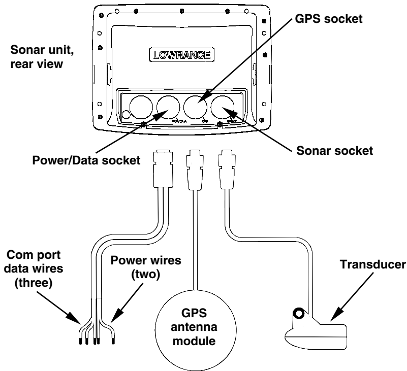
Cable connections.
