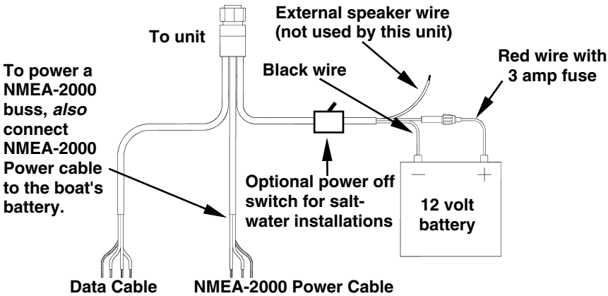
Power connections for the LMS-480 series sonar/GPS unit.
