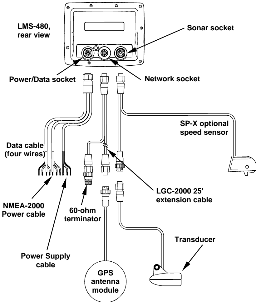
LMS-480 cable connections.
