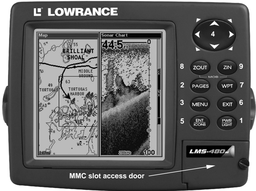
LMS-480 series sonar/GPS unit, front view, showing map with sonar split screen, keyboard and access door for the MMC slot.
