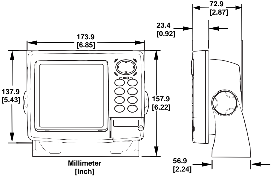
Front view (left) and side view (right) showing dimensions of LMS-480 sonar/GPS unit when mounted on gimbal bracket.
