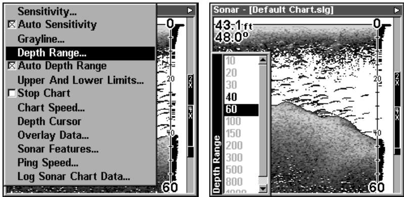
At left, Sonar Page menu with Depth Range command selected. At right, the Depth Range Control Scale.
