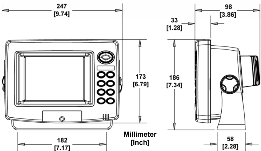
Front view (left) and side view (right) showing dimensions of the GlobalMap 7200 and GlobalMap 7300 mounted on gimbal brackets.
