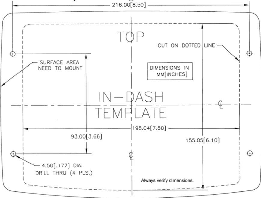
In-dash mounting template for the GlobalMap 7200 and GlobalMap 7300, showing dimensions. The figure above is not printed to scale.
