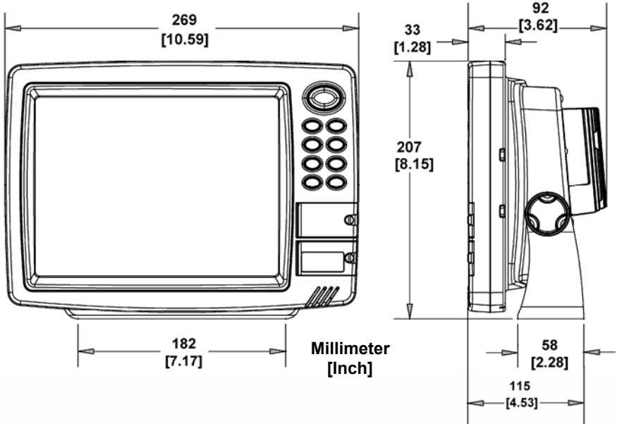
Front view (left) and side view (right) showing dimensions of the GlobalMap 8200c and GlobalMap 8300CHD mounted on gimbal brackets.
