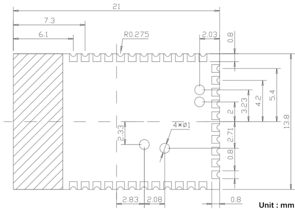
MK05 PCB land pads(TOP View)
