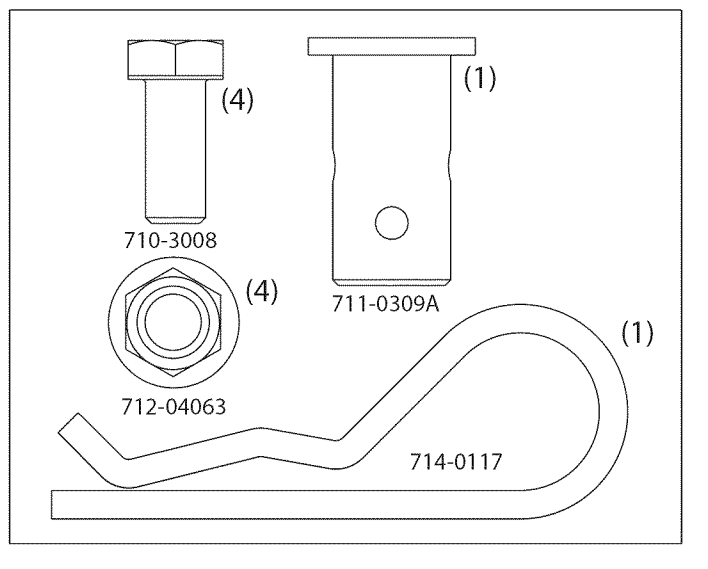
Hardware Pack for 689-00087
