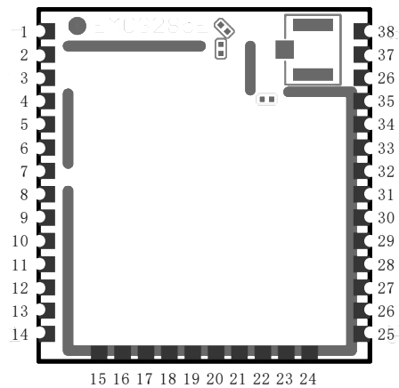
Figure 3 EMC3285 Pin Arrangement
