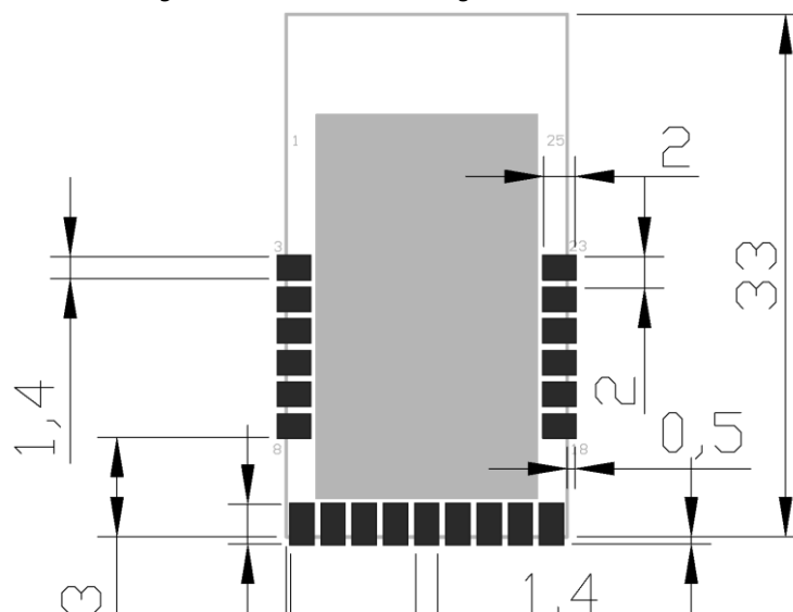
Figure 15 EMC3280 PCB Package size (unit: mm)
