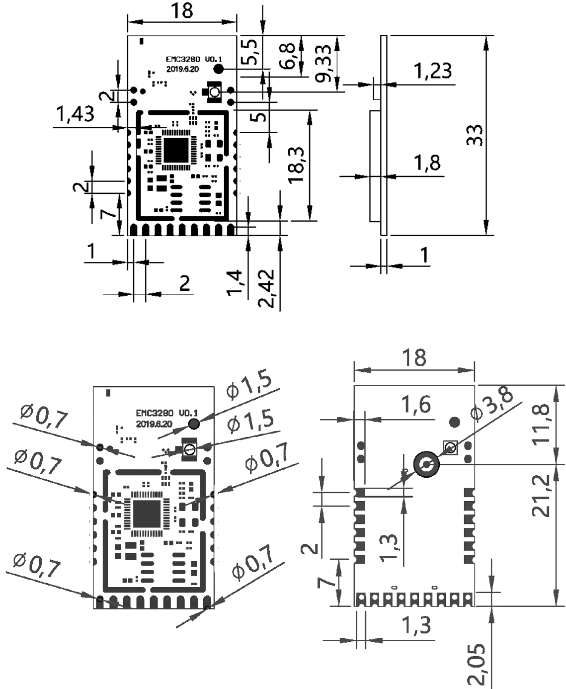
Figure 13 EMC3280 three view (unit: mm, error: \pm 0.1 )
