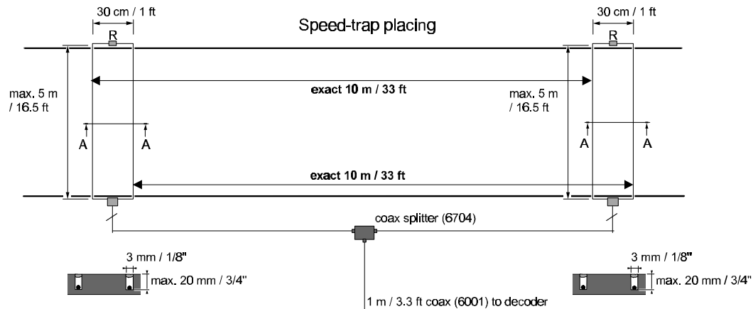
Loop installation for speed trap setup.
