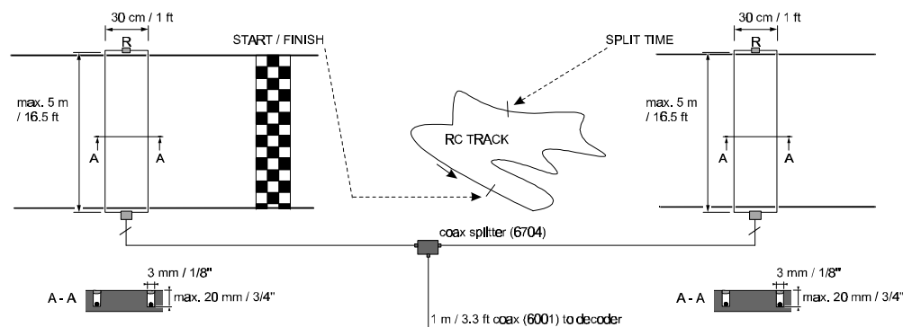
Loop installation for split time setup
