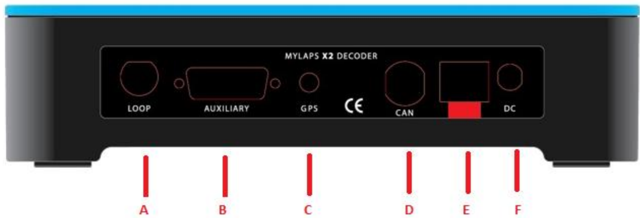
Figure 1.2 Connections of the decoder
