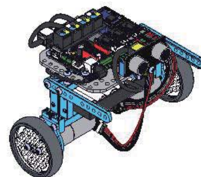
Self-Balancing Robot
