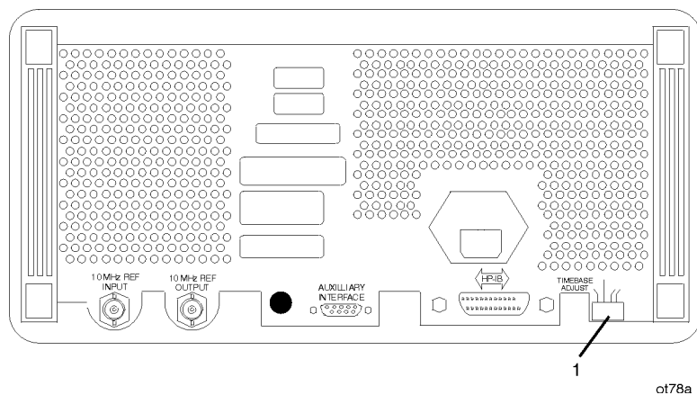
Figure 7-1. Timebase Adjust Switch Location
