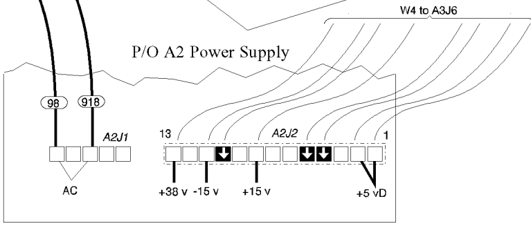
Bottom View with Motherboard Cover Removed
