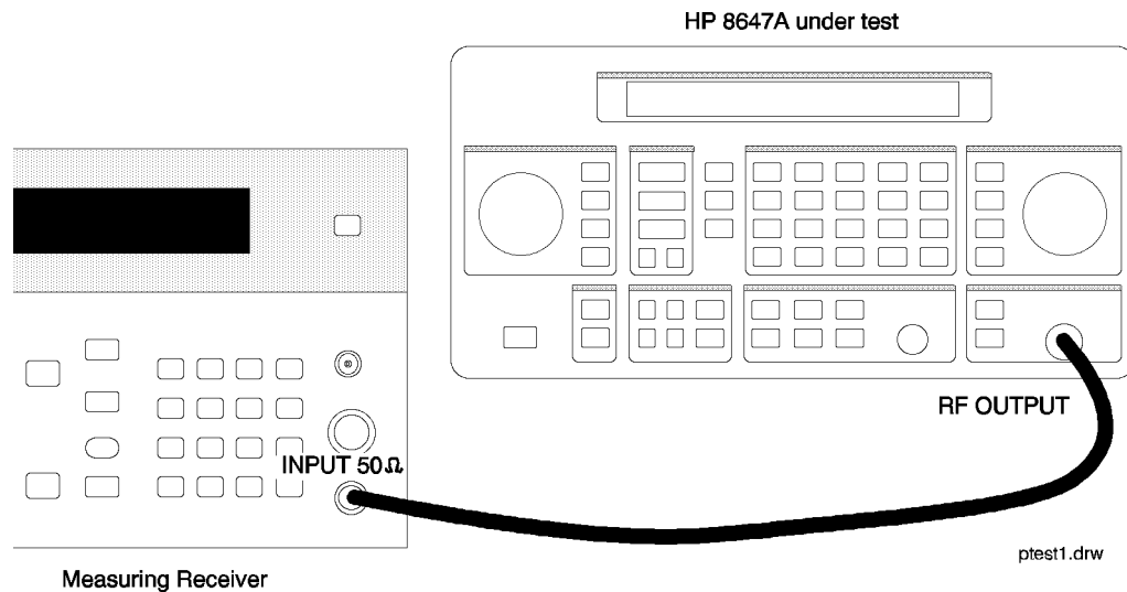
Figure 8-5. Phase Modulation Accuracy Equipment Setup
