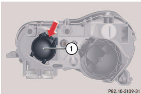
1 Housing cover for high beam flasher bulb, parking and standing lamp
