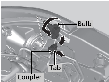
Coupler
