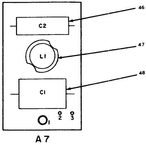
Figure 5. Rejection amplifier.
