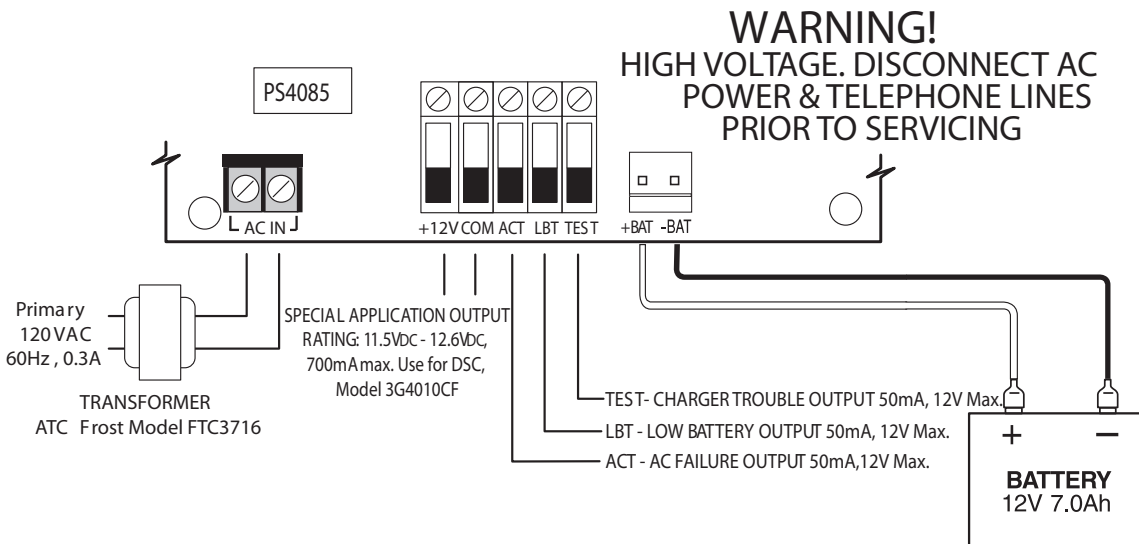
Figure 12-3 Power Supply Wiring Diagram
