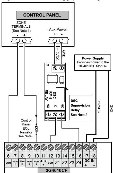
Figure 12-5 Power Supply and Supervision Wiring Diagram
