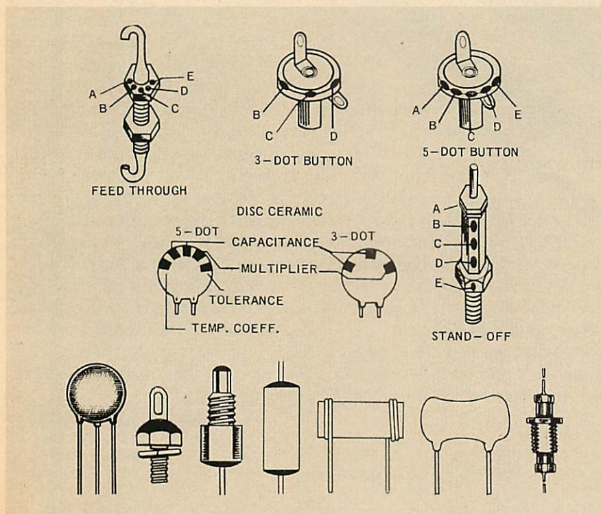
Fig. 11—Capacitors are available in a tremendous variety of sizes, shapes and styles. The letters adjacent to the capacitors indicate color-coded dots which supply data.
