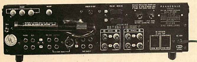
Fig. 2—Rear panel.
