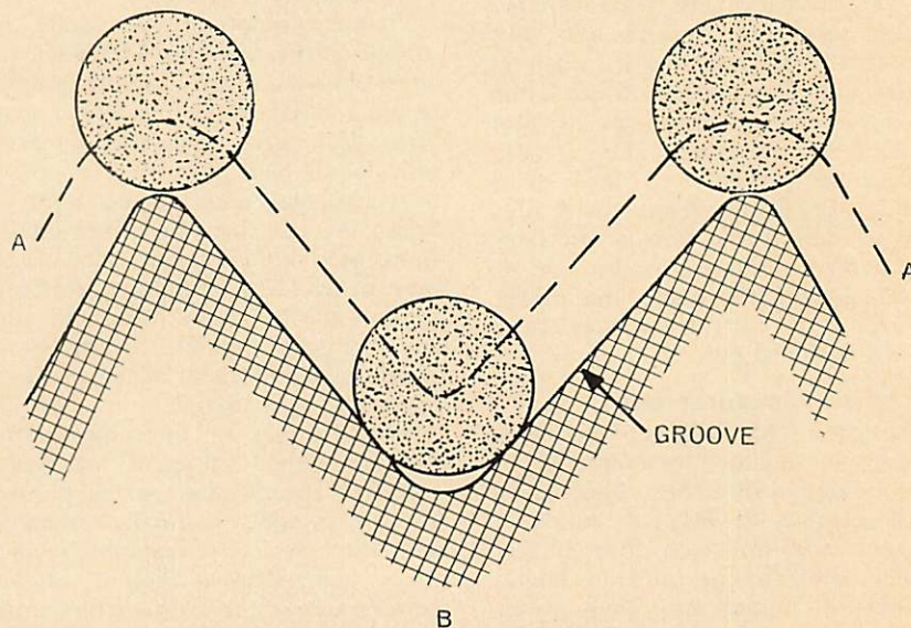
Fig. 2—How tracing distortion is caused. A-A is the stylus path.
