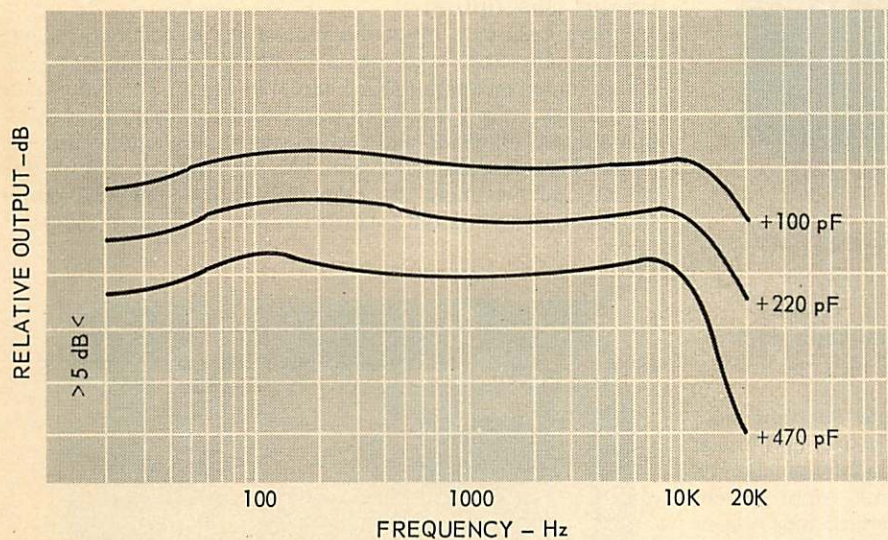
Fig. 4—Showing effect of lead capacity.
