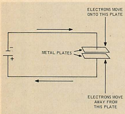
Fig. 2 —Electrons move from the negative terminal of the voltage source to one of the metal plates of the capacitor. An equal number of electrons leave the other plate and move to the positive terminal of the battery. This electron displacement charges the capacitor.
