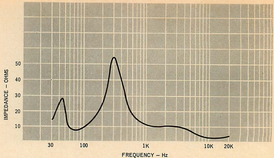
Fig. 4—Impedance characteristics.
