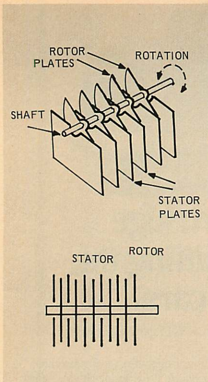
Fig. 10 —A variable capacitor consists of a number of fixed plates, all connected, called the stator. The rotor plates are mounted on a shaft which can be turned.
