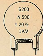
Fig. 8—If the surface area is large enough, the data is printed directly on the body of the capacitor.
