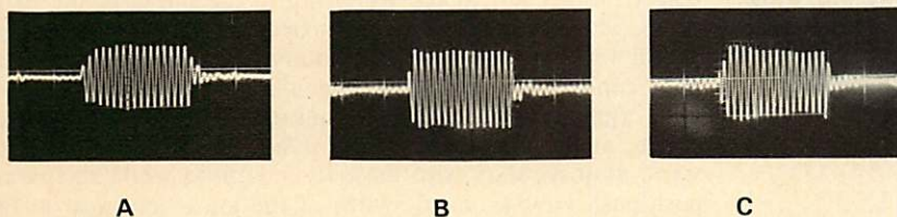
Fig. 2—Tone burst characteristics at A, 50; B, 1000, and C, 5,000 Hz.
