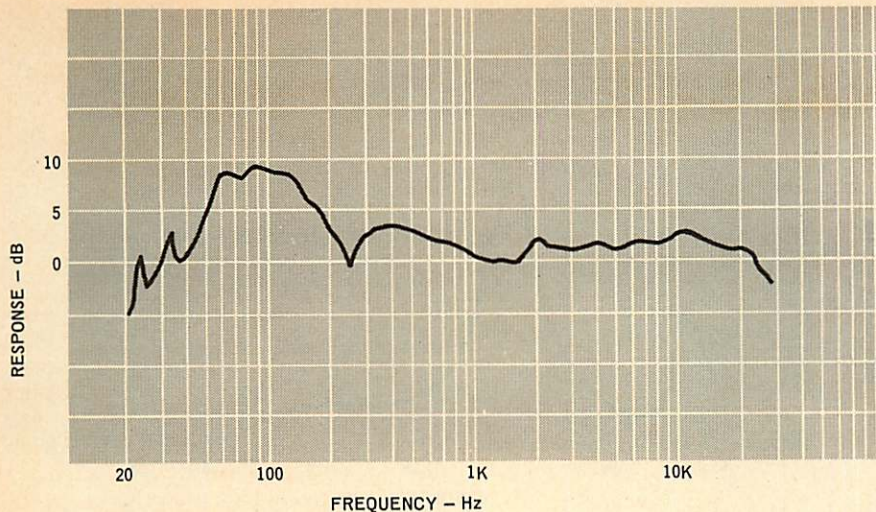
Fig. 1—Frequency response
