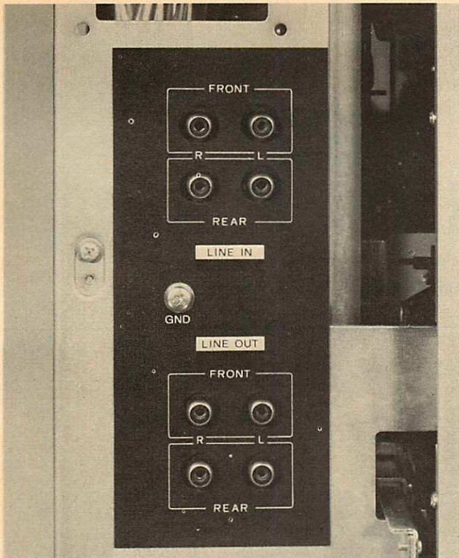
Fig. 2—Input panel.
