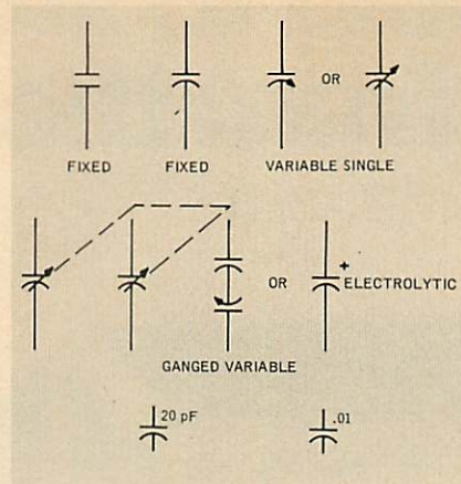
Fig. 12—Capacitor symbols.
