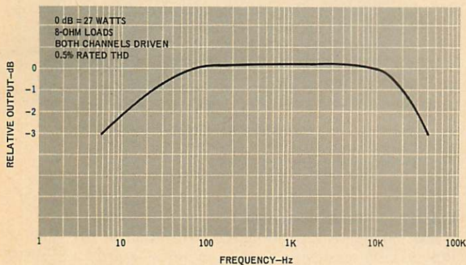
Fig. 6—Power bandwidth.
