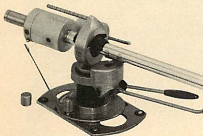
Fig. 5—Anti-skating device as used in the SME arm.
