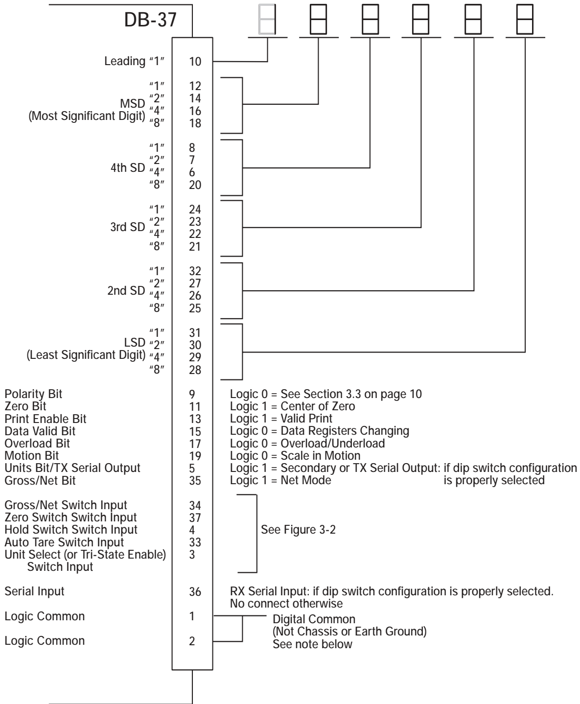
Figure 3-1. BCD External Connection
