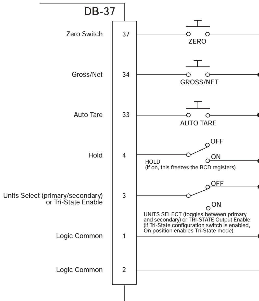
Figure 3-2. BCD Remote Switches
