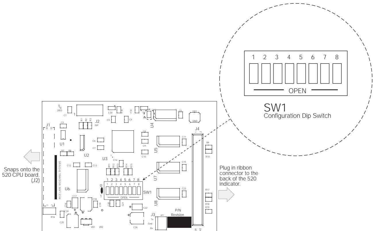
Figure 2-3. BCD Option Card
