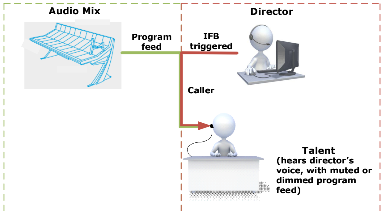
Figure 4-26 Broadcast scenario with IFB trigger
