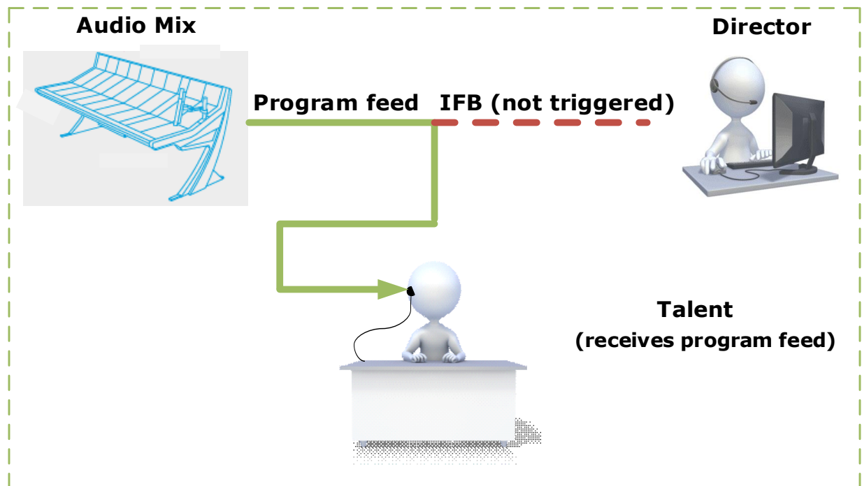
Figure 4-25 Broadcast scenario with no IFB trigger.
