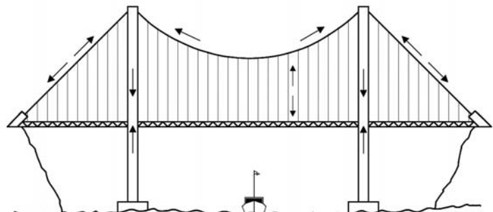
Forces acting on a suspension bridge.
