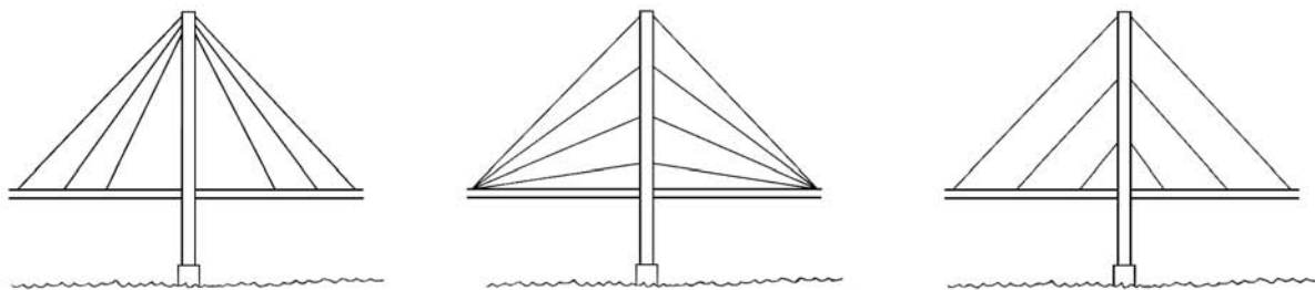
Fig. 47 - Cable designs.
