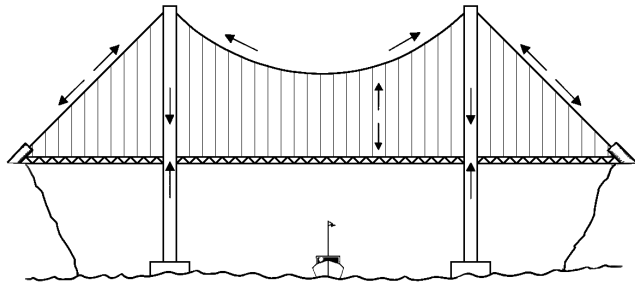
Fig. 50 - Forces acting on a suspension bridge.
