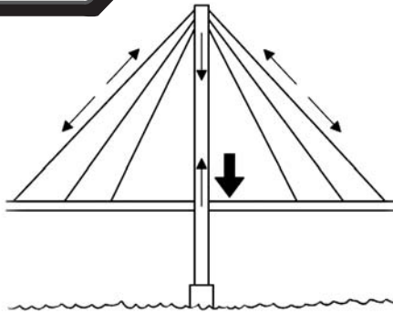
Fig. 46 - Forces acting on a cable-stayed bridge.
