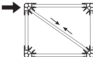
Fig. 25 - Compression acting on the strut.
