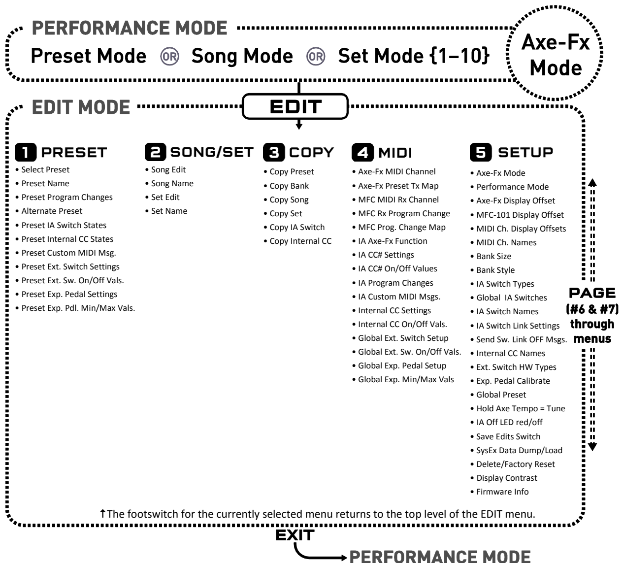
Figure 1-6: Software Map
