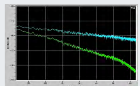
LEFT: Output of real-time noise analysis software, showing the noise attenuation curve of a standard AC noise filter. Note the uneven shape of the curve (the green line).
