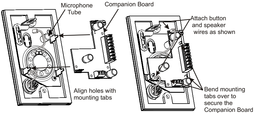
Completed Sub-assembly
