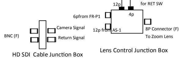
HD SDI Cable Junction Box
