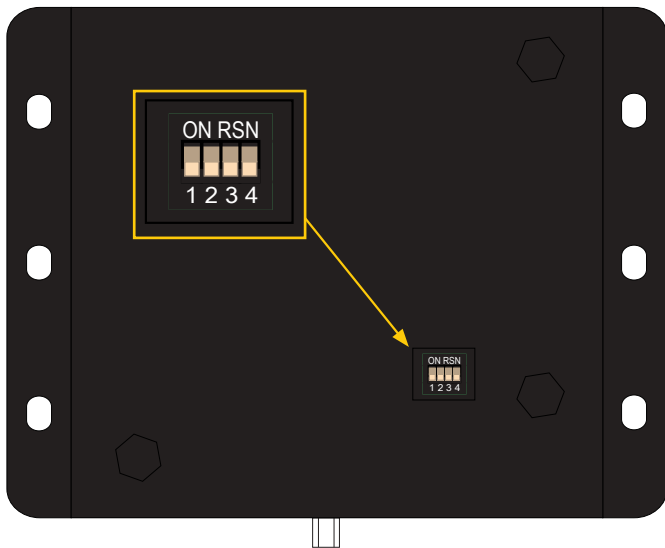
Sender unit
