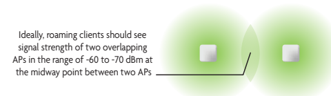
XAP-1410 Multiple AP Coverage and Overlap
