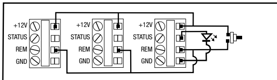
Fig. B - Three M-8S units configured for Parallel Momentary mode with LED indicator.
