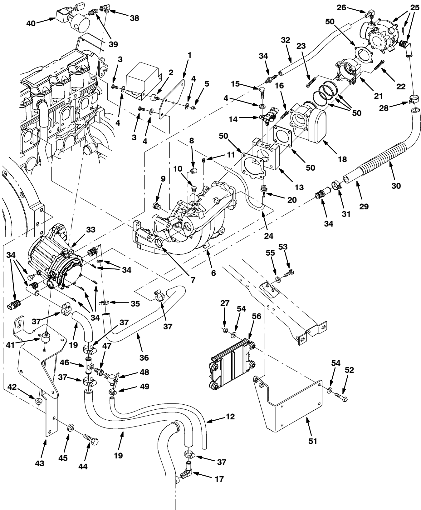
Fig. 17 - Engine EFI and Vaporizer Group, LPG (009000- )
