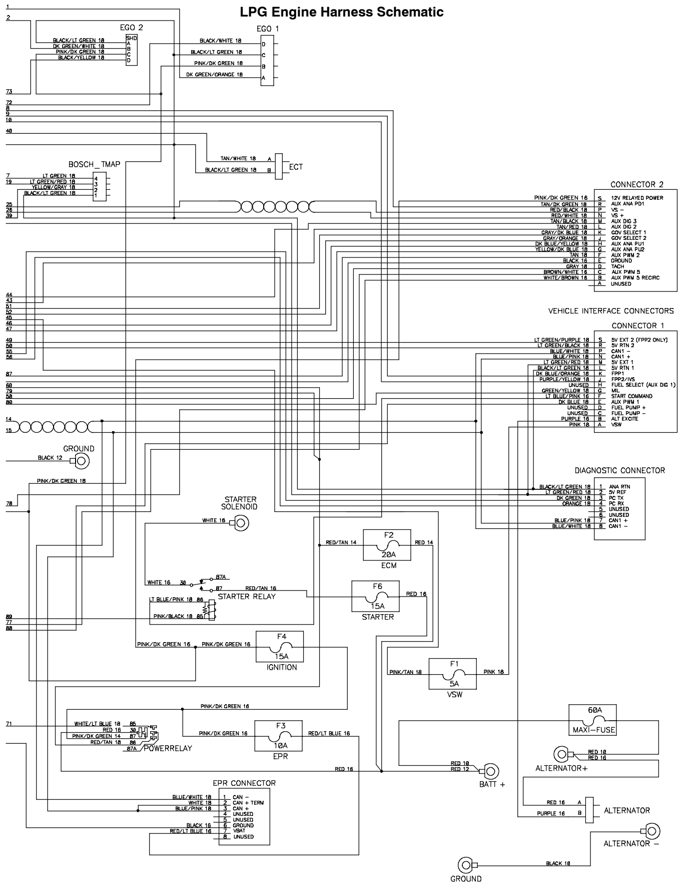
Fig. 49 - Electrical Schematic (009000- )
