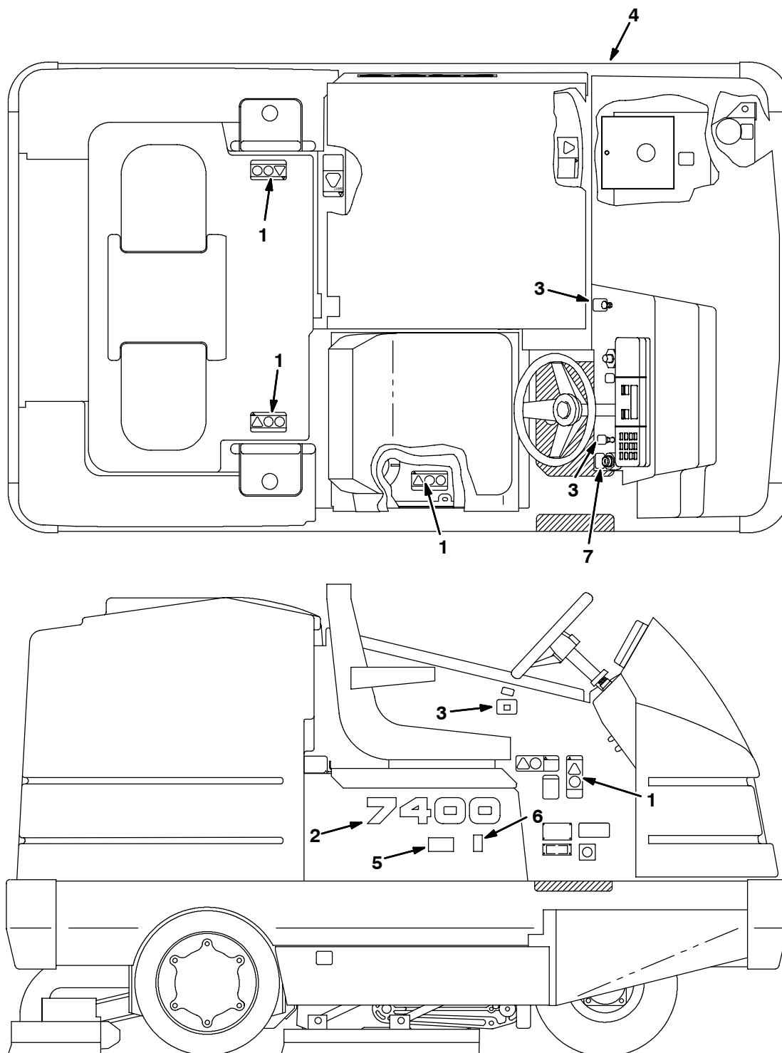
Fig. 67 - Label Group
