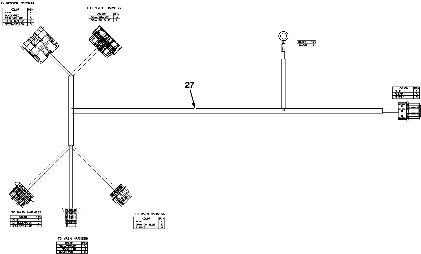
Fig. 50 - Electrical Wire Harnesses Group
