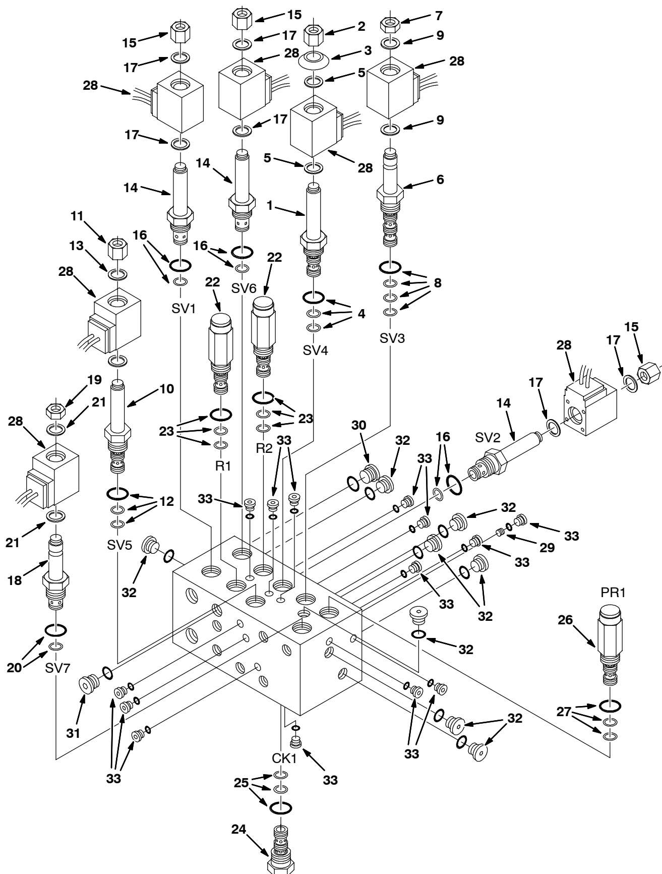
Fig. 8 - Hydraulic Solenoid Valve Breakdown, Side Brush and Nylon Brush, 71762
