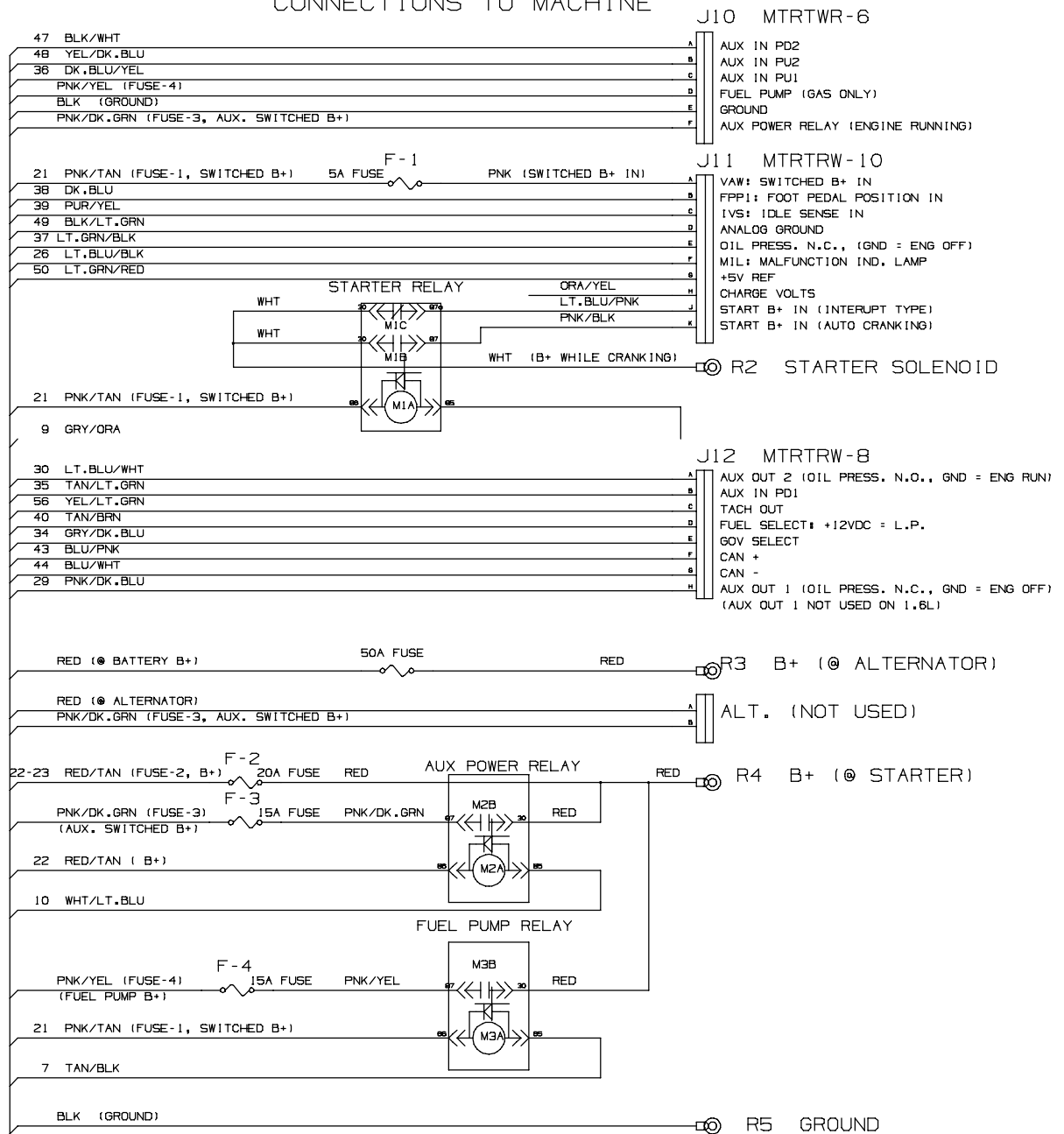
Fig. 48 - Electrical Schematic (007000-008999)
