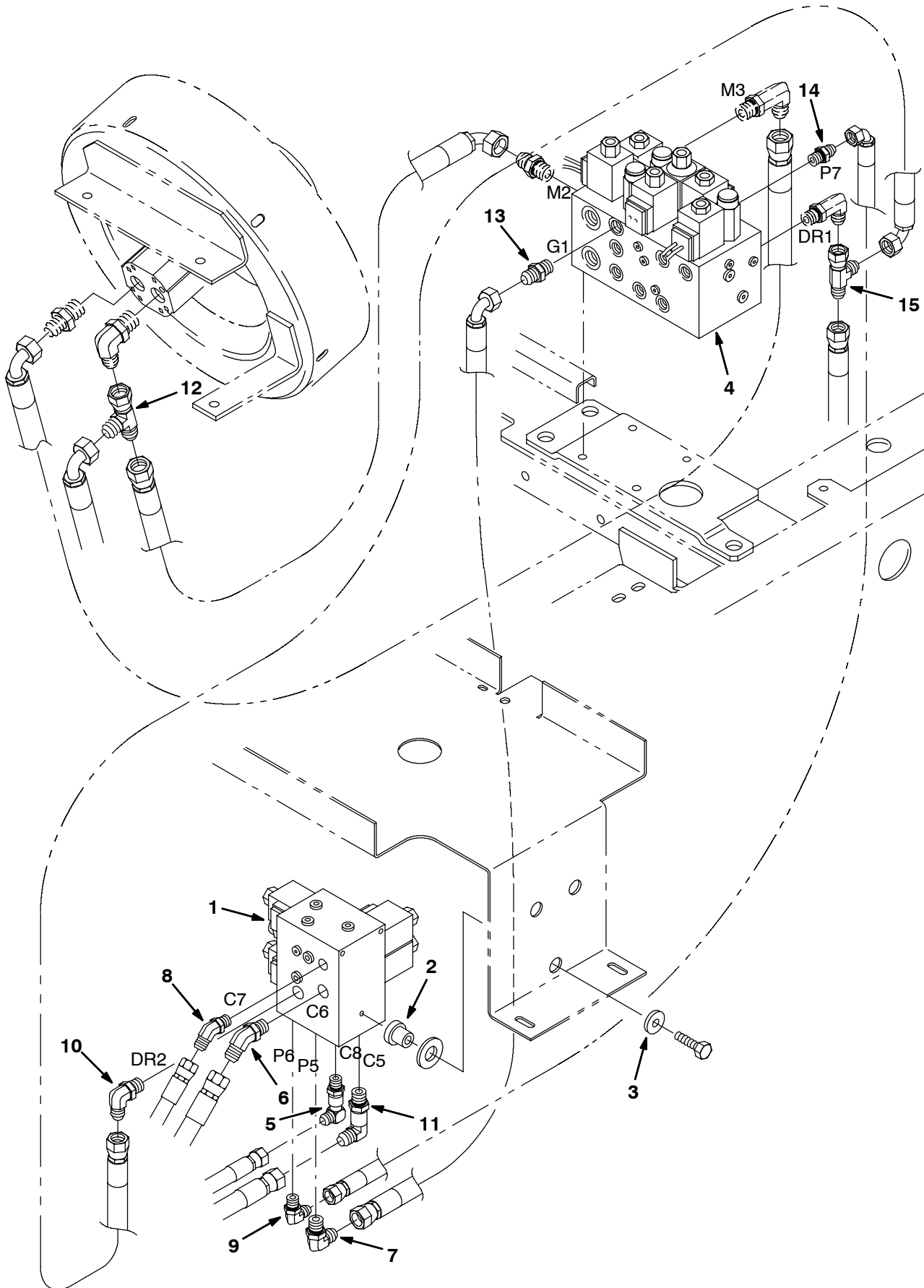
Fig. 11 - Side Brush Hydraulic Group
