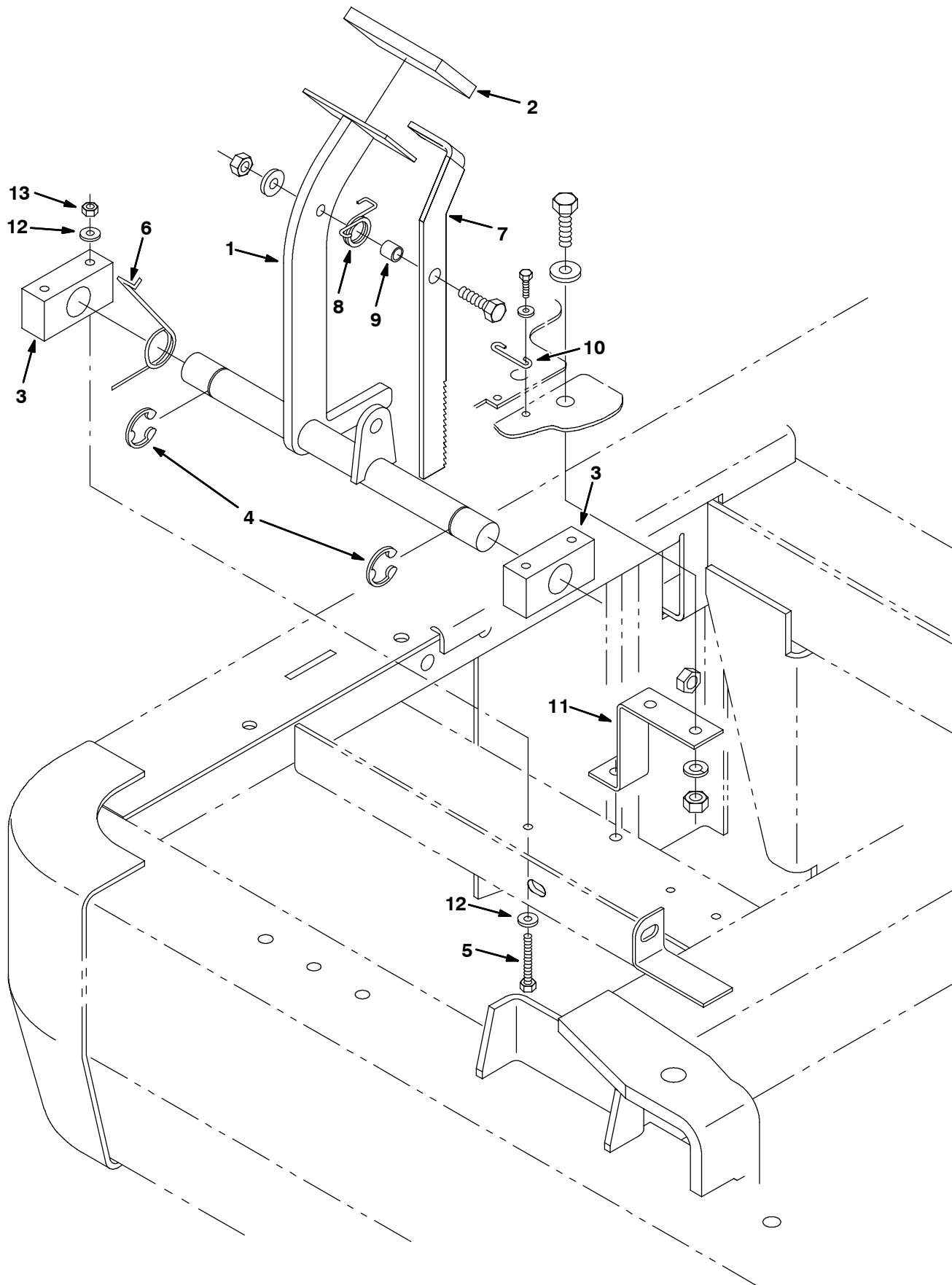
Fig. 33 - Brake Pedal Group
