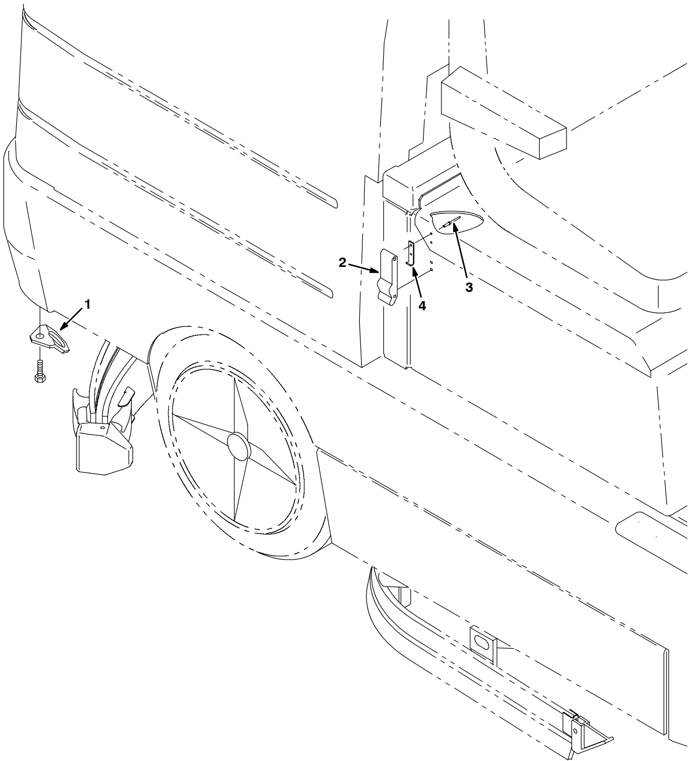
Fig. 29 - Transport Group
