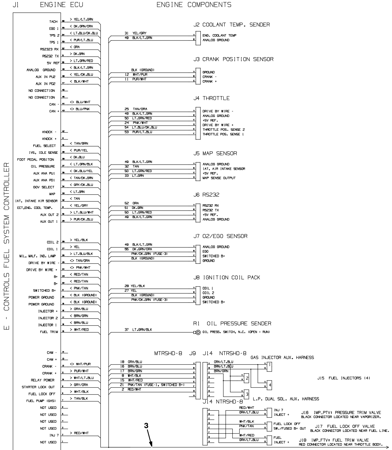
Fig. 50 - Electrical Wire Harnesses Group ENGINE COMPONENTS
