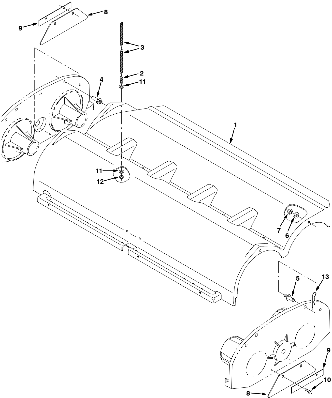
Fig. 52 - Scrub Brush Housing Group
