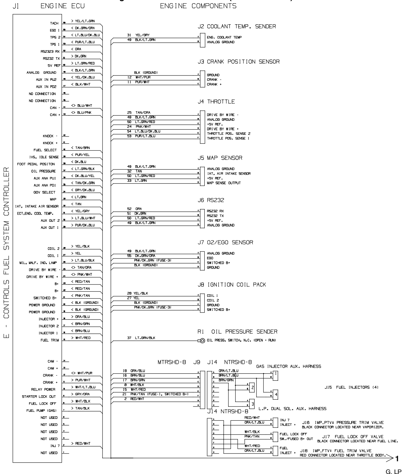
Fig. 48 - Electrical Schematic (007000-008999)
