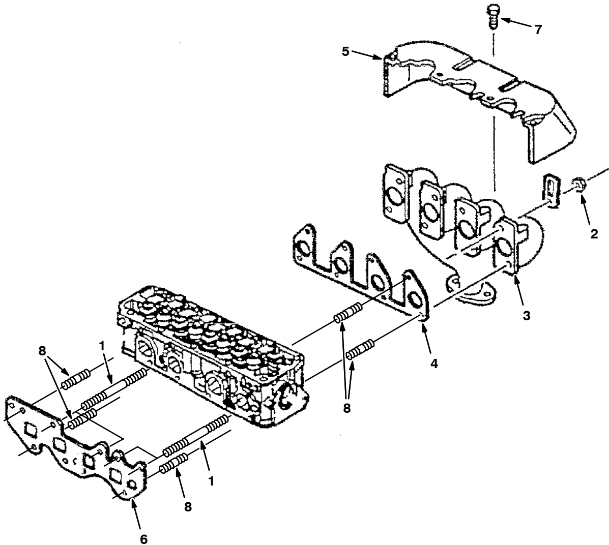
Fig. 5 - Manifold Group
