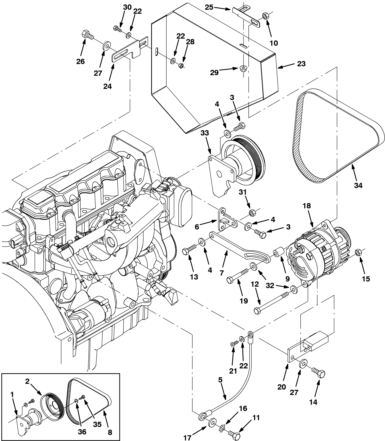
Fig. 22 - Engine Alternator Group
