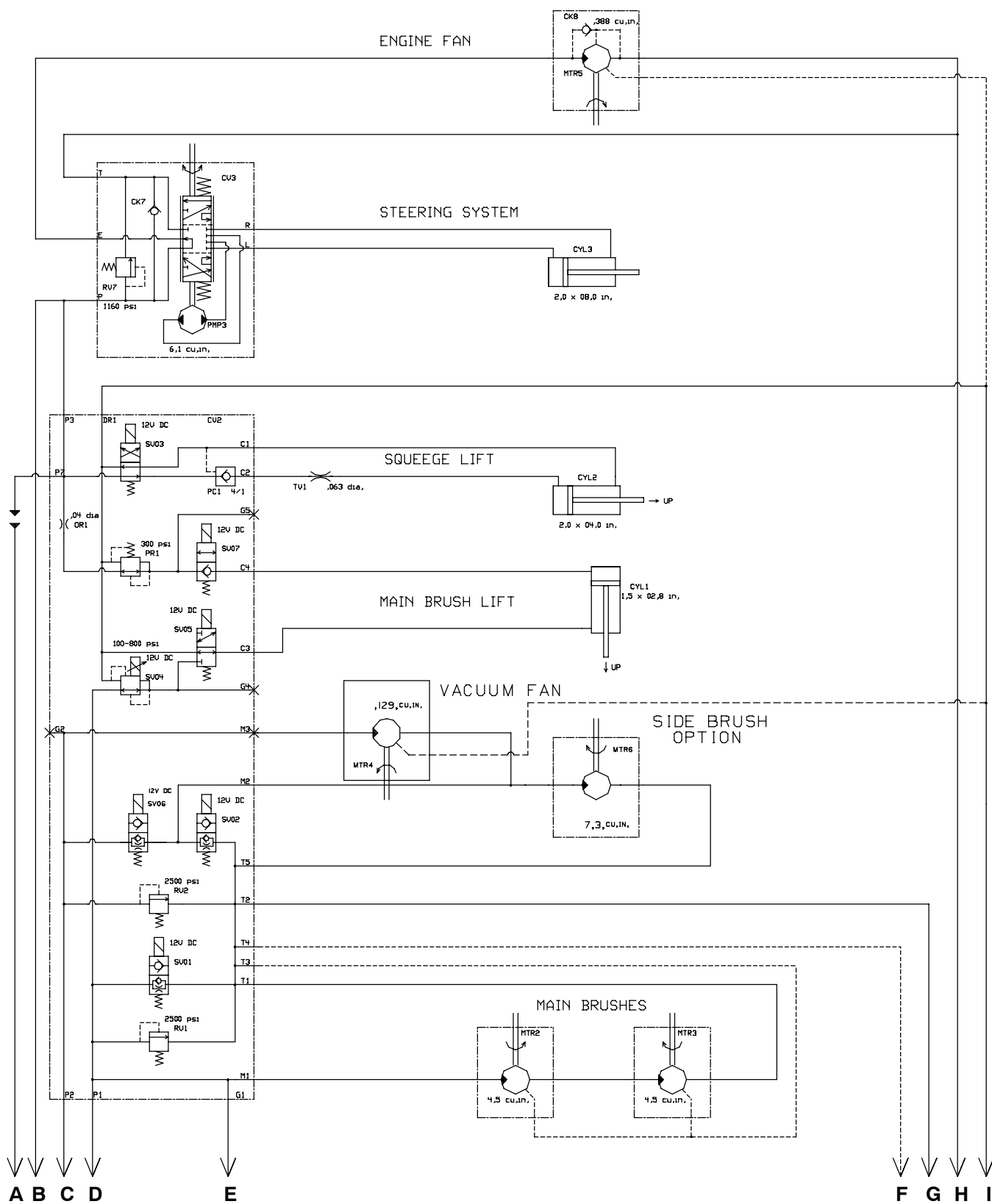
Fig. 41 - Hydraulic Schematic
