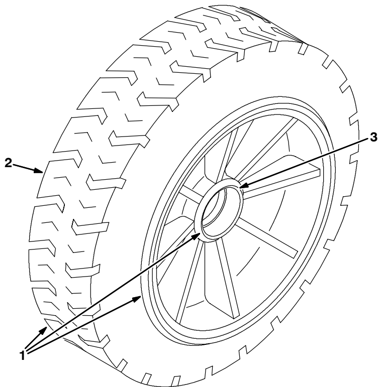
Fig. 24 - Solid Non Marking Turf Tire and Wheel Assembly
