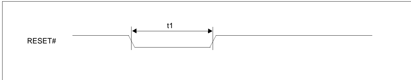
Figure 6-2 SID13A04 RESET# Timing
