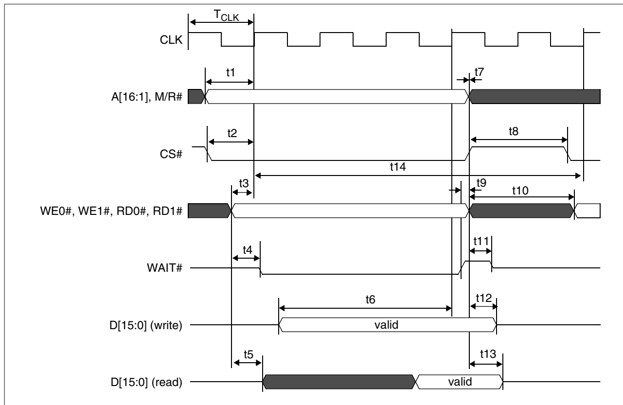
Figure 6-3: Generic #1 Interface Timing
