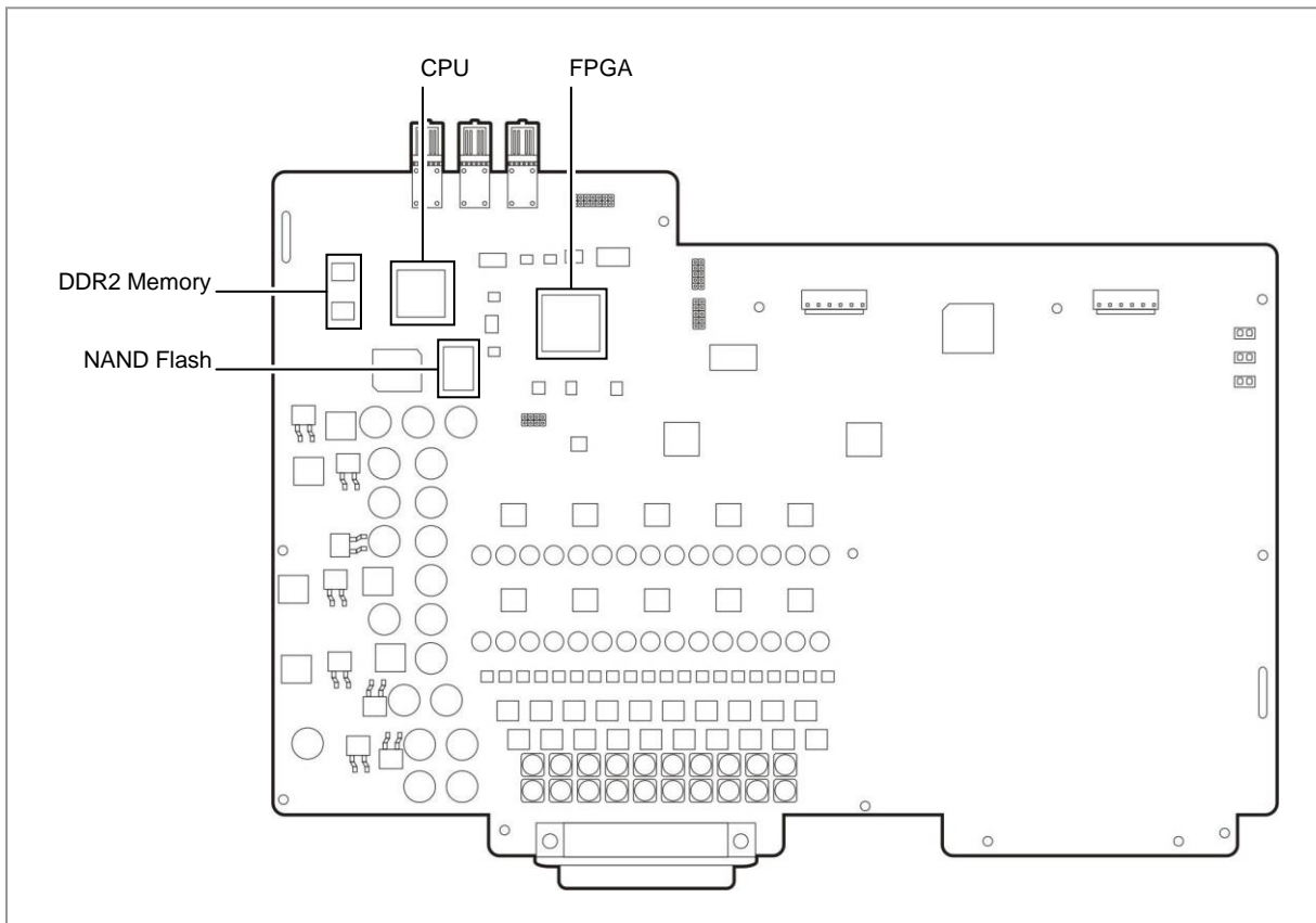
Figure 61. 20FXS Board
