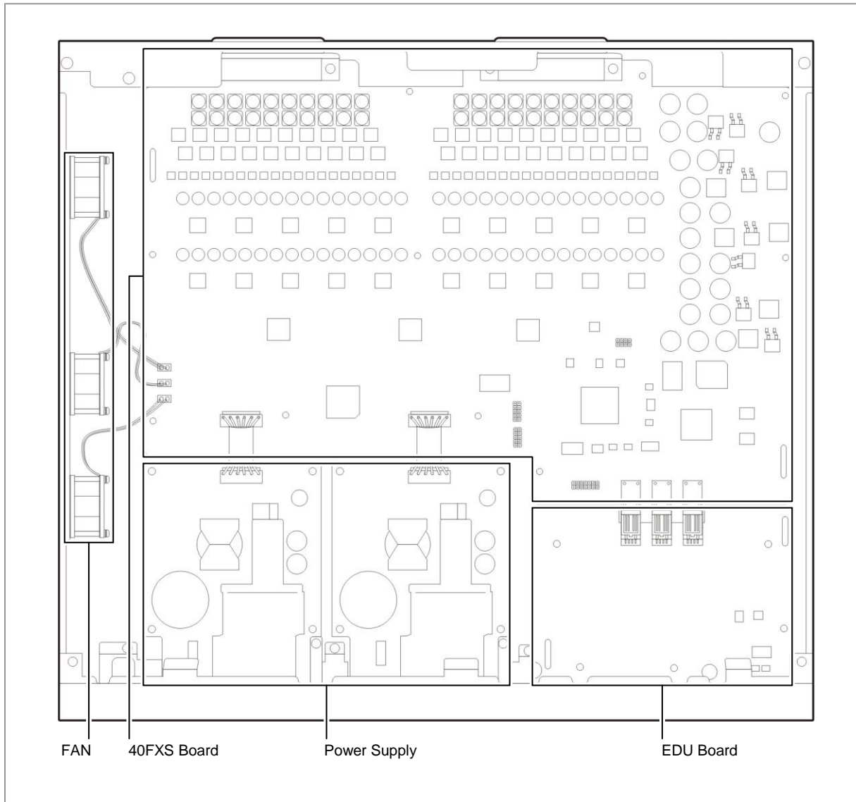
Figure 64. IPX-G540S Interior
