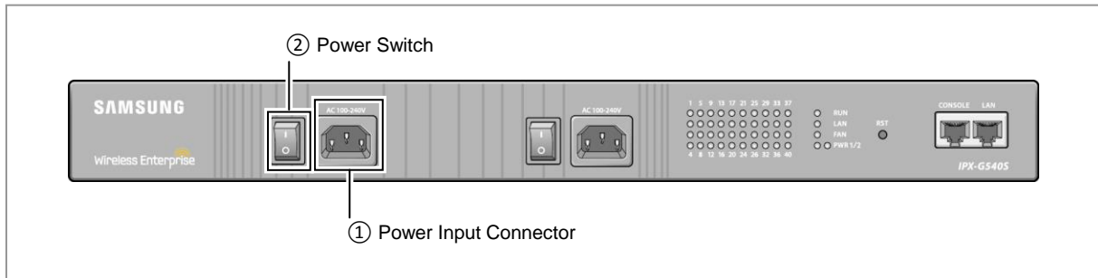
Figure 67. IPX-G540S Power Input
