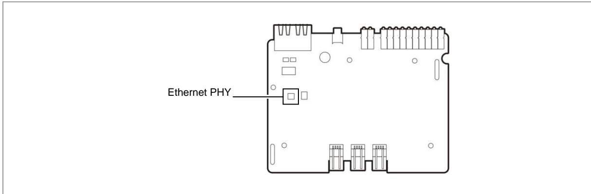
Figure 60. EDU Board
