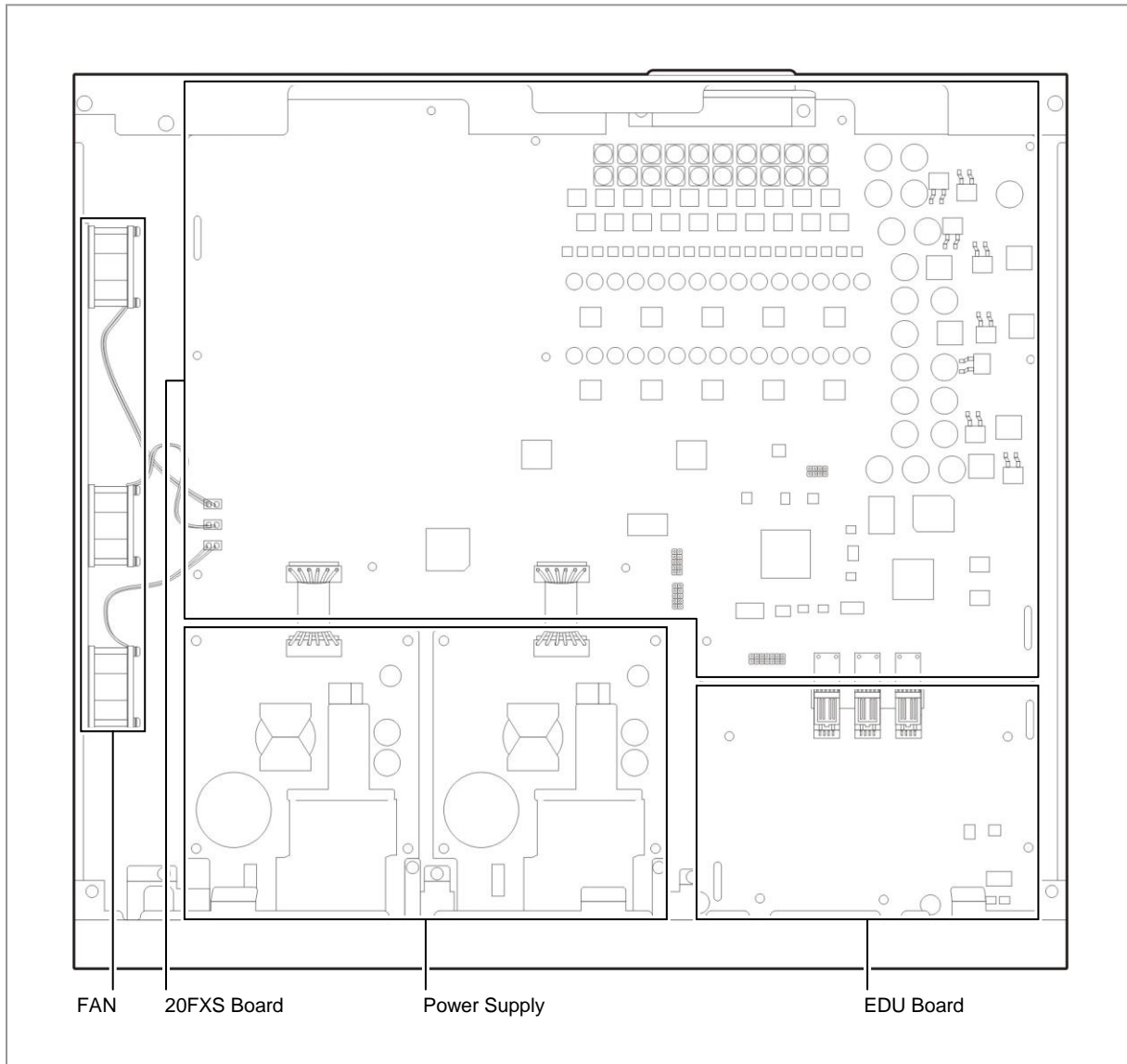
Figure 59. IPX-G520S Interior
