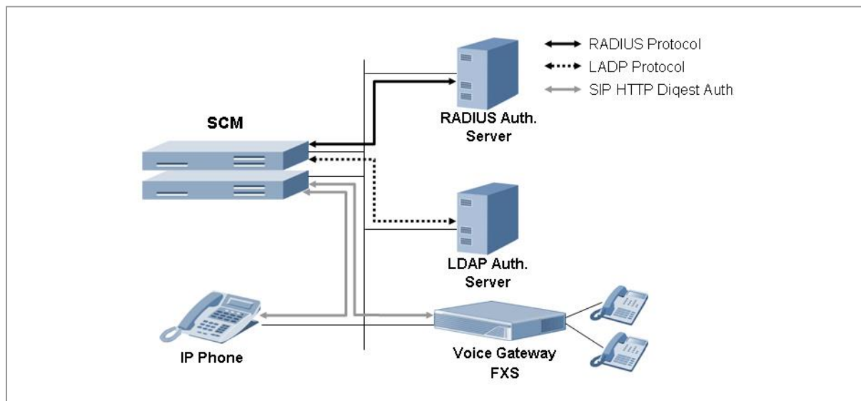
Figure 74. User Authentication
