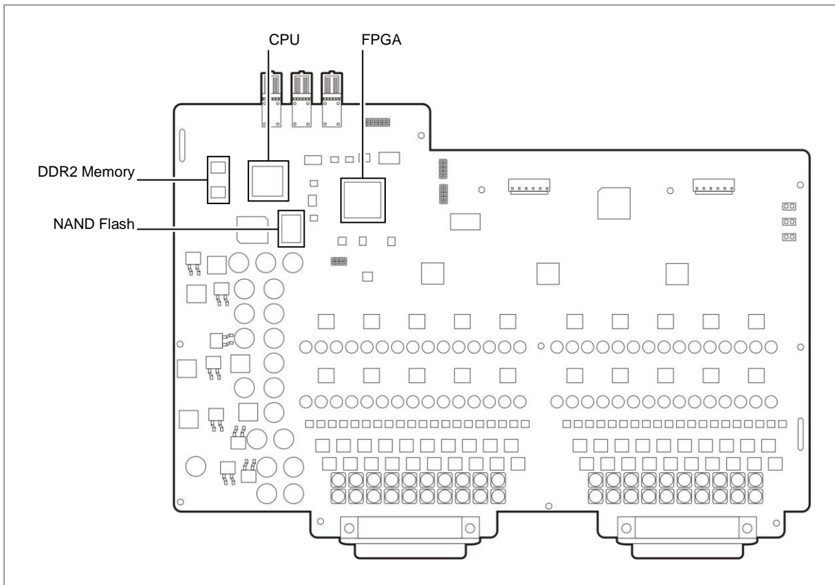
Figure 66. 40FXS Board
