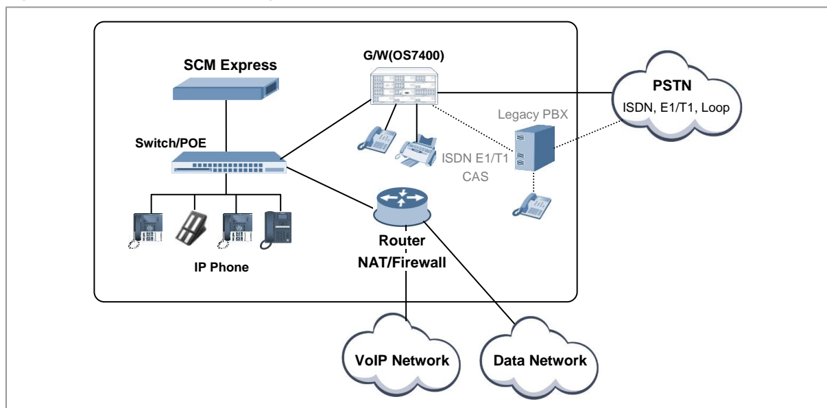
Figure 2. Active-Along SCM Configuration Example
