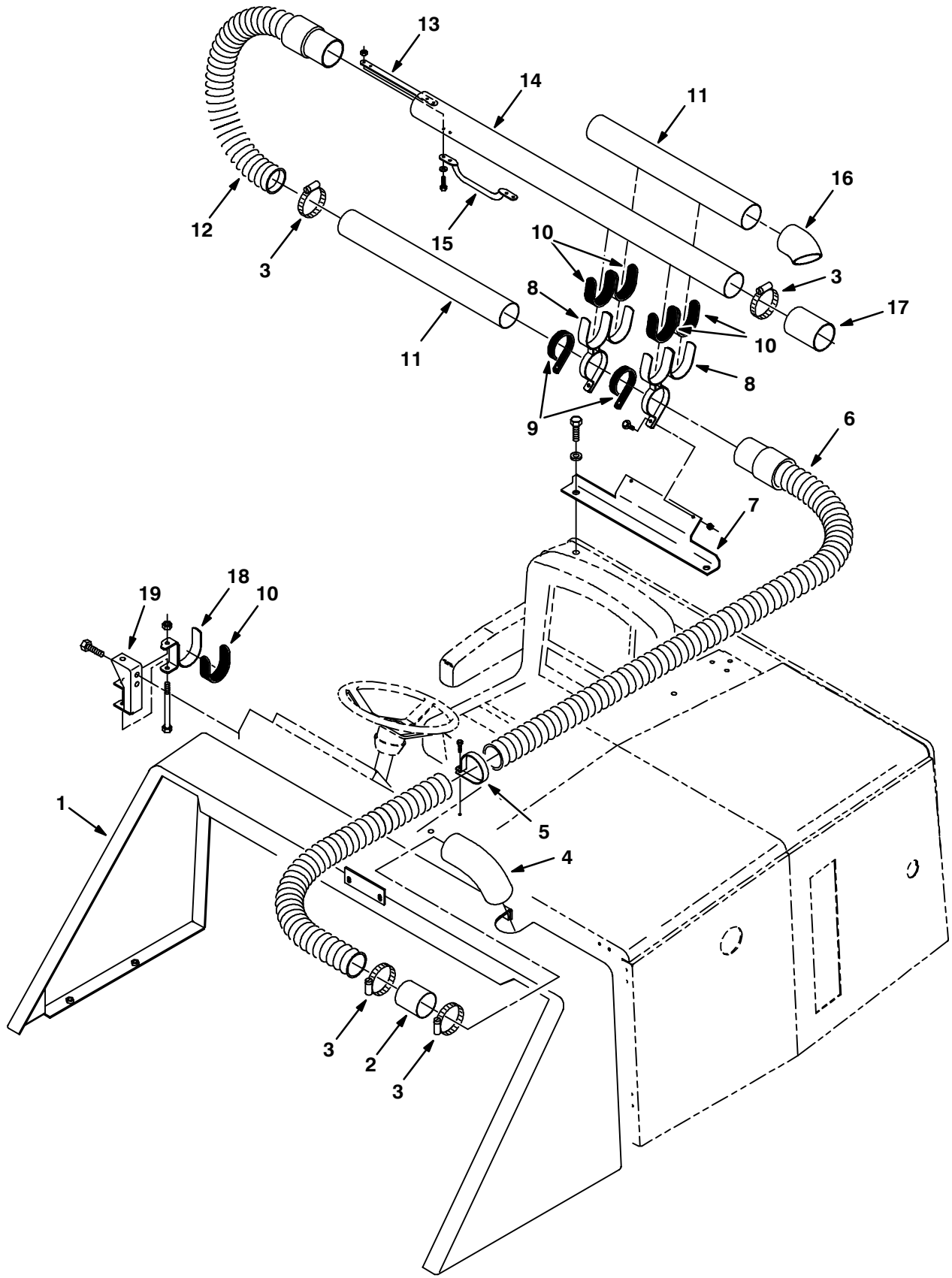
Fig. 12 – Blower Group
