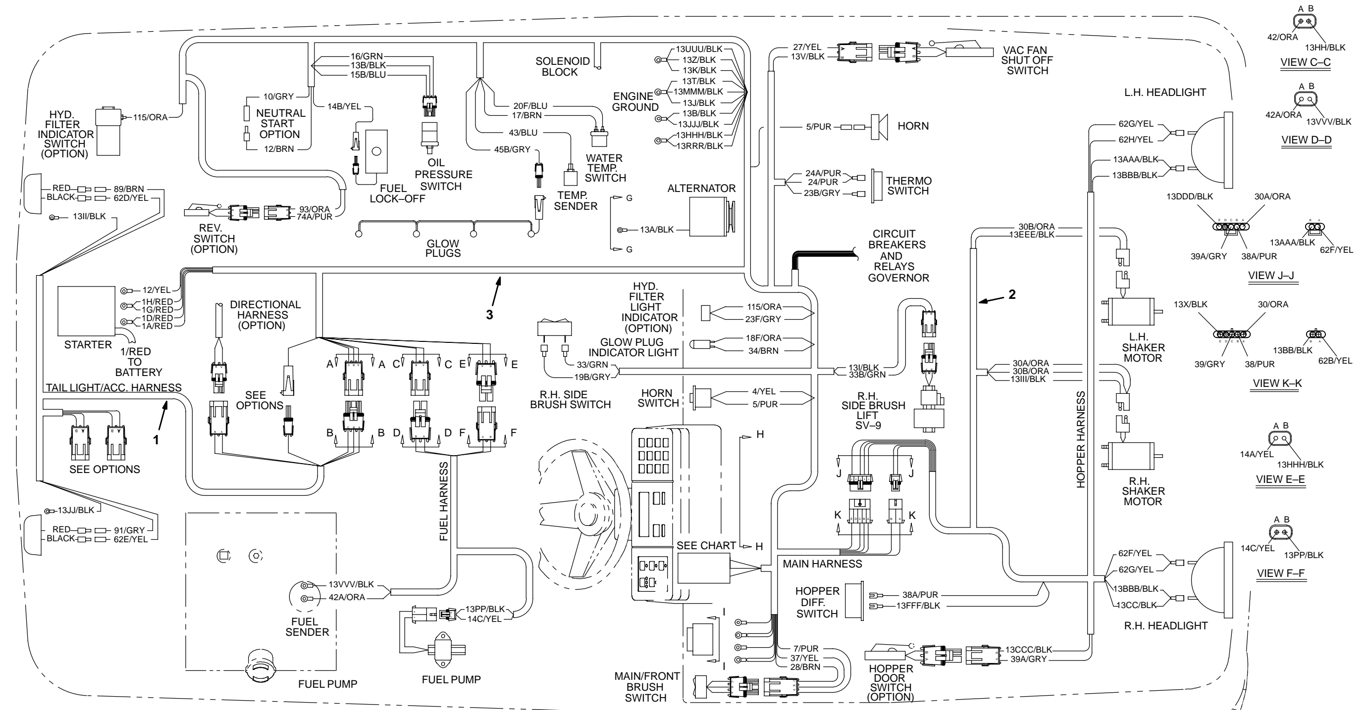
Fig. 71 – Wire Harness Group
