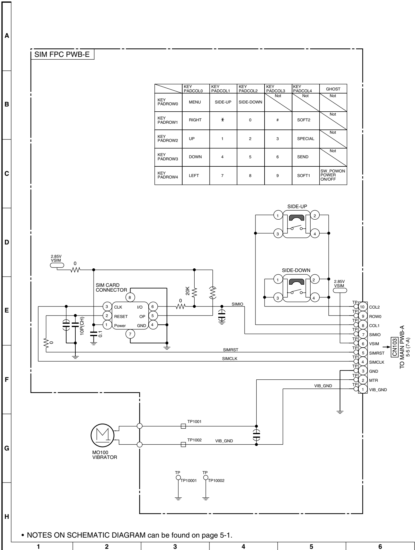
Figure 9 SCHEMATIC DIAGRAM (5/6)
