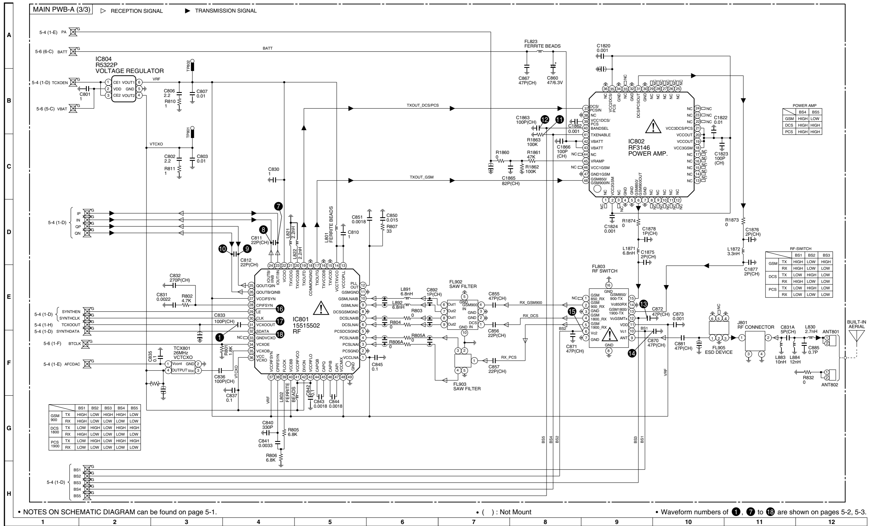
Figure 3 SCHEMATIC DIAGRAM (3/6)
