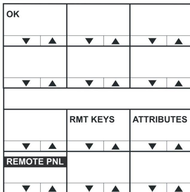
Figure 6-59: Remote panel menu (RMT keys and attributes mode) for desktop panels
