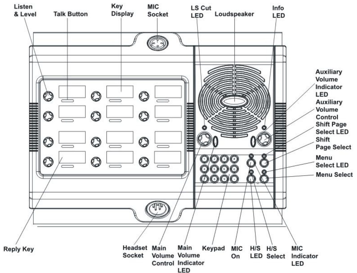
Figure 3-12: V12RDD front panel lights and controls
