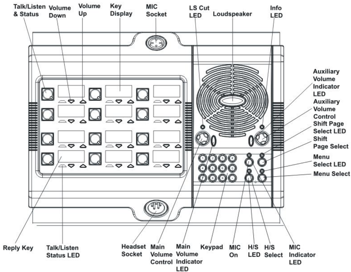
Figure 3-11: V12PDD front panel lights and controls
