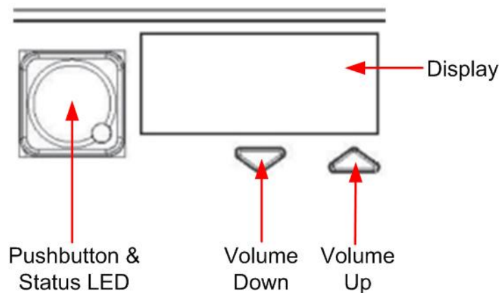
Figure 3-16: Pushbutton key display window controls
