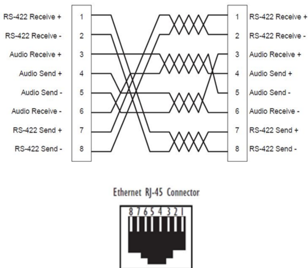
Figure 4-26 Pinouts for RJ-45 crossover cable
