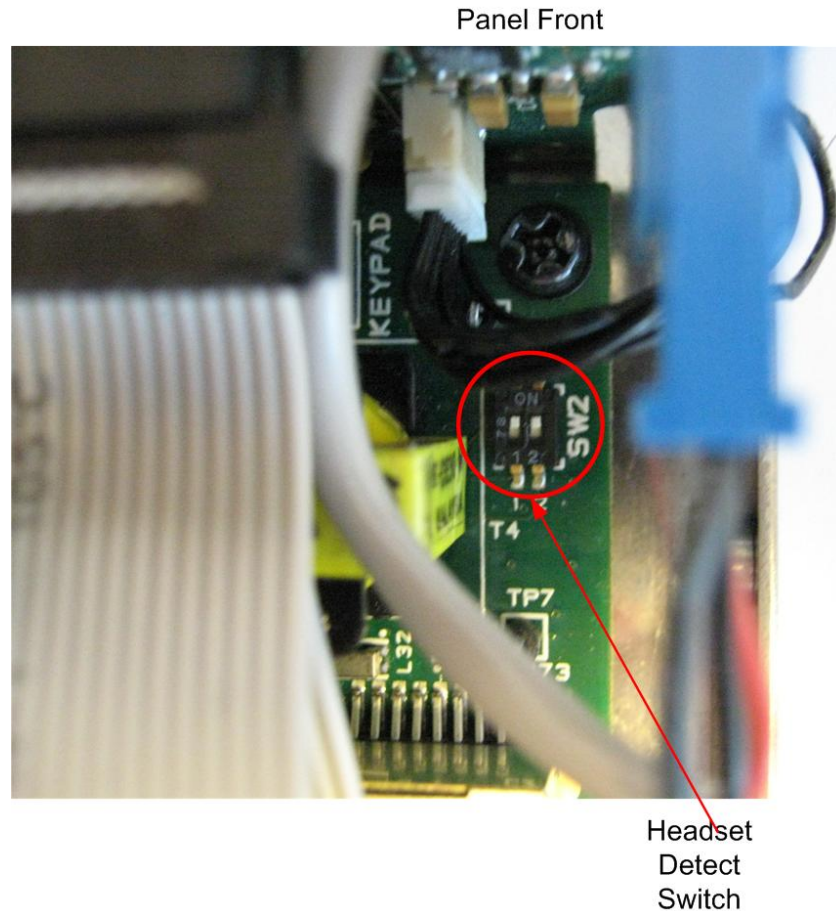
Figure 4-35: DIP switch location (headset detect)
