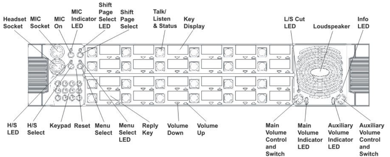
Figure 3-5: V24PD front panel lights and controls
