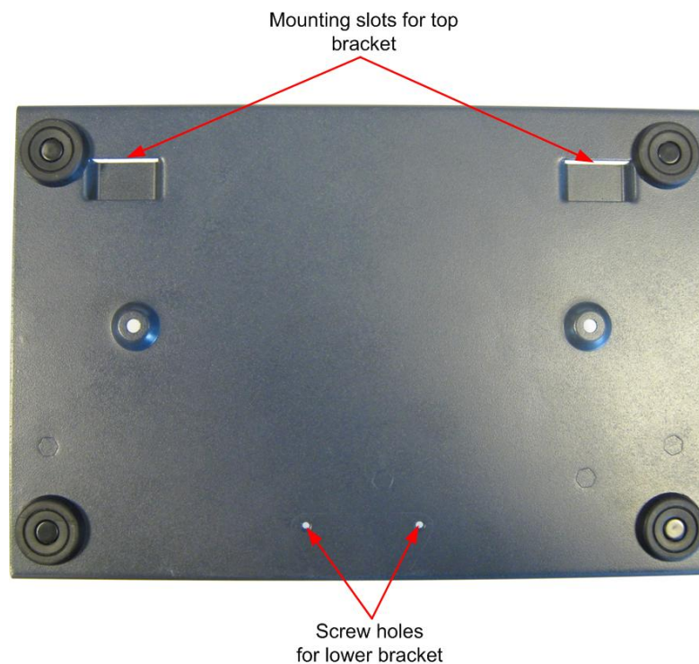
Figure 4-4: Desktop casing (without lower bracket)
