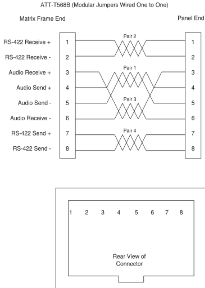
Figure 4-14: Matrix to panel wiring (analog)
