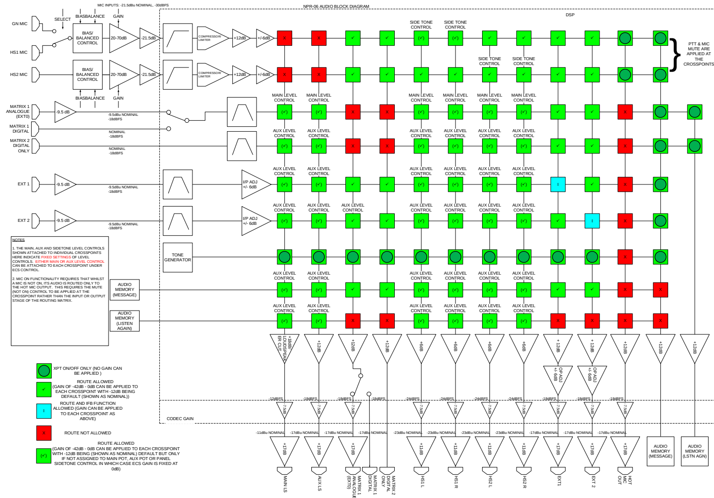
Figure 5-4: V-Series audio block diagram
