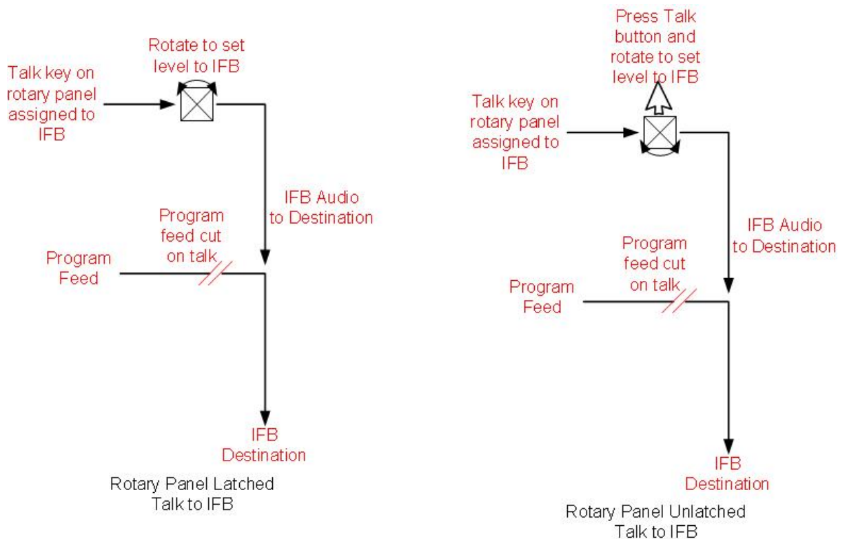
Figure 5-3: Rotary Panel latched and unlatched talk to IFB
