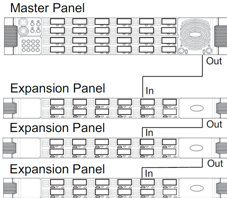
Figure 4-22: Example of daisy chained panels
