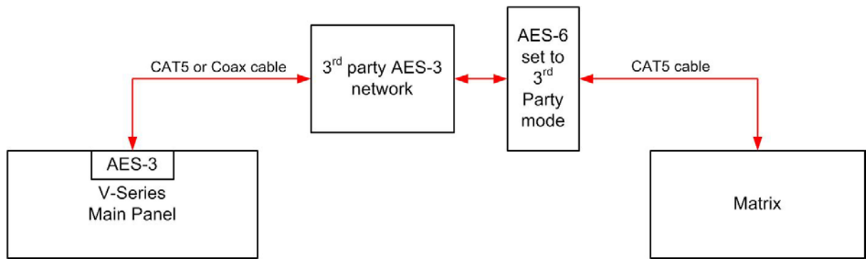
Figure 4-19: Panel connected by 3 rd party AES-3 network
