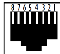
LAN Port Ethernet RJ-45 Connector
