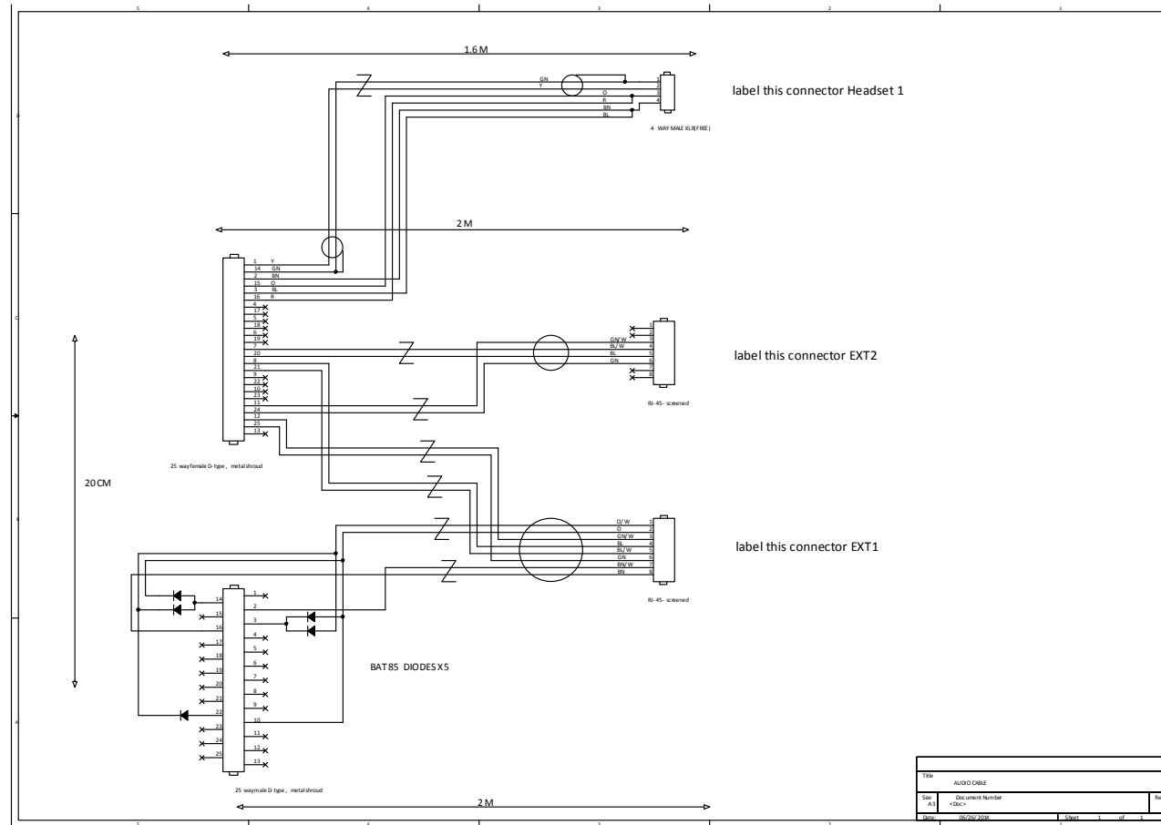
Figure 4-29 Pinout diagram for cable harness
