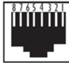
Figure 4-26 Pinouts for RJ-45 crossover cable
