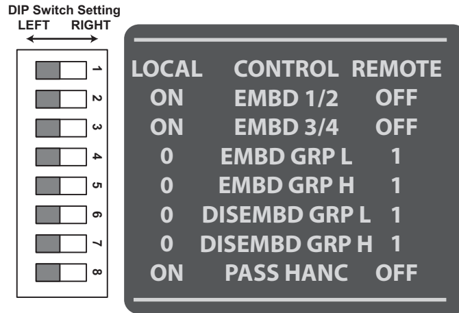
Figure 1. DIP Switches
