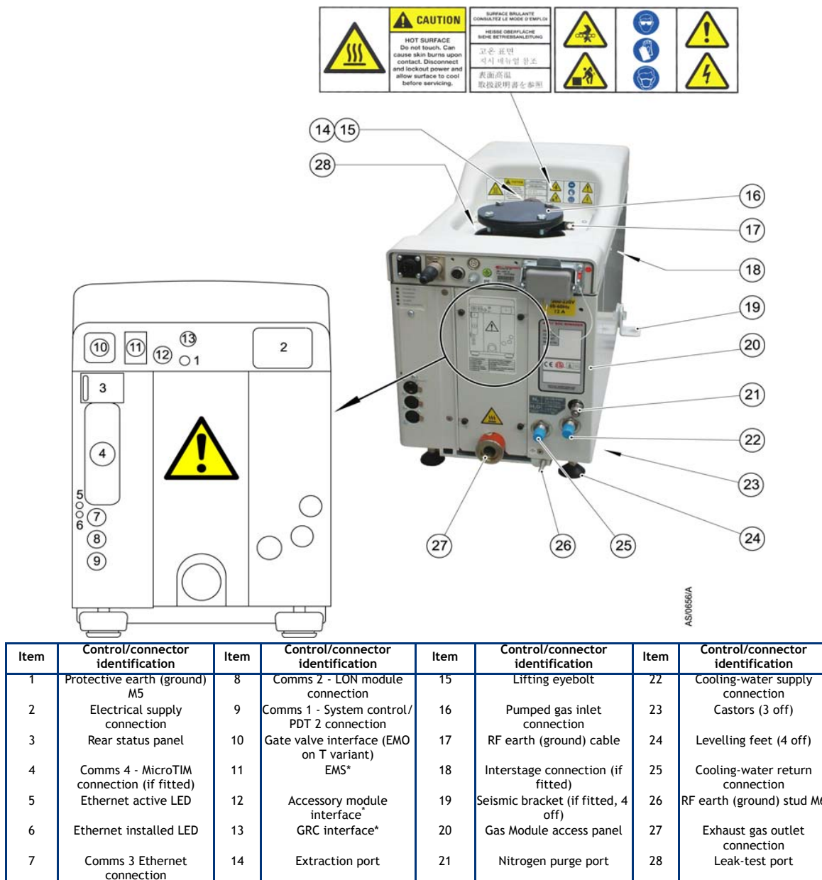
Figure 2 - The controls/connectors
