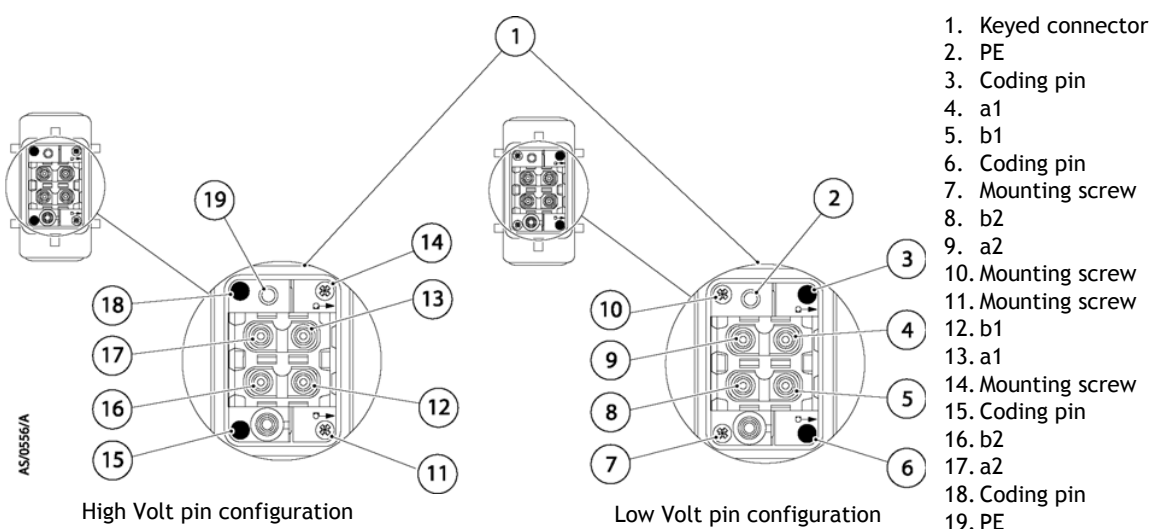
Figure 8 - High and low volt coding pin arrangement
