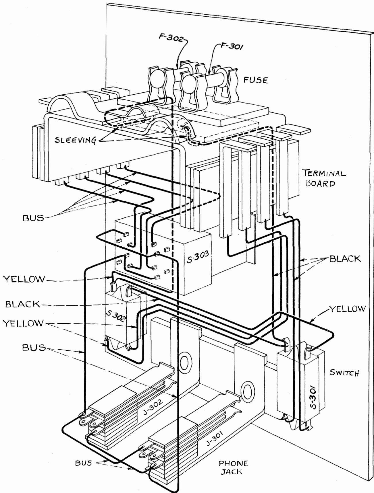
Figure 21—Connection Diagram. Control Unit CRV-23073 (P-714101)
