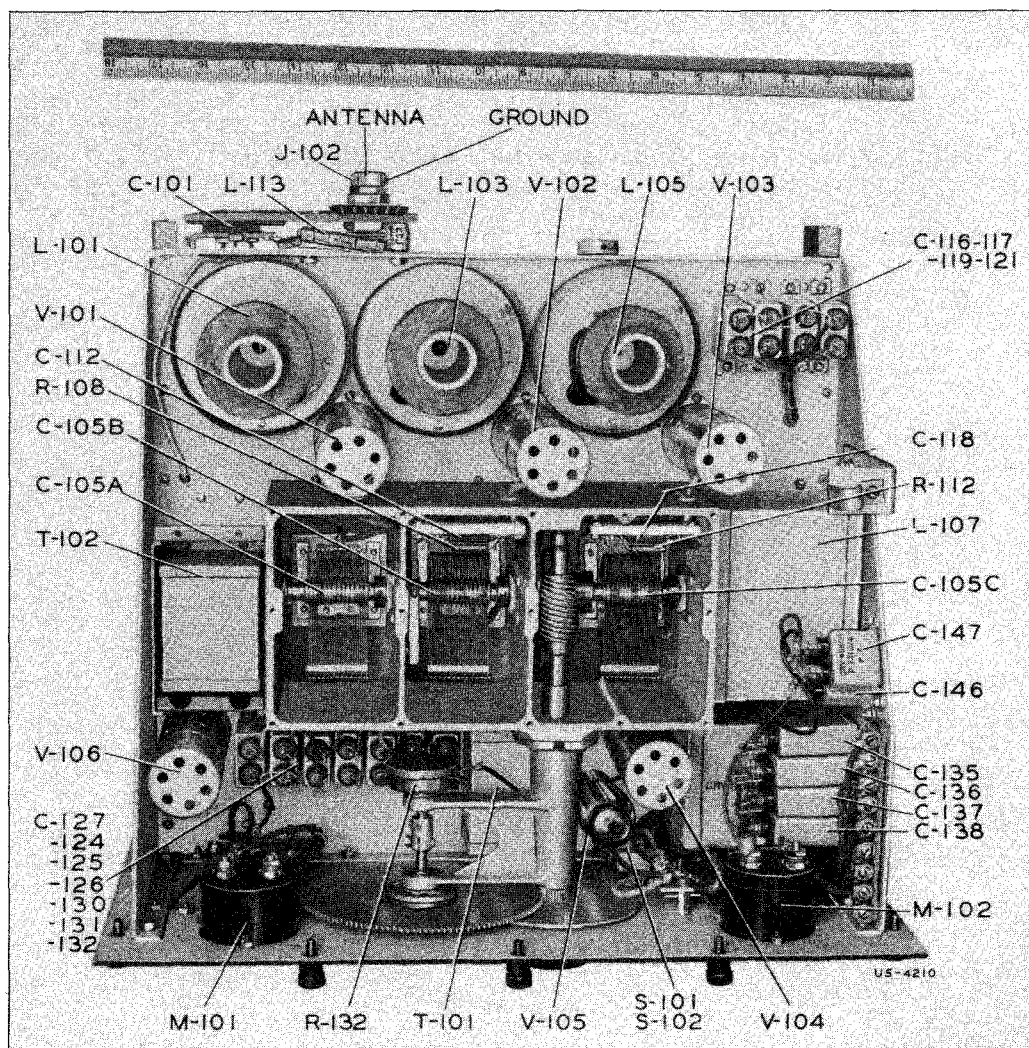
Figure 3—Receiver Unit CRV-46155 (Top View of Chassis—Covers Removed)
