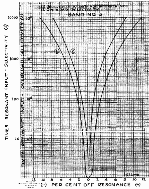
Figure 11—Average Selectivity and Overload Selectivity (1) Selectivity to 100% Mod. Interference; (2) Overload Selectivity
