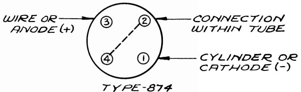
Figure 22—Tube Socket Connections (K-850992-Sub. 3)
