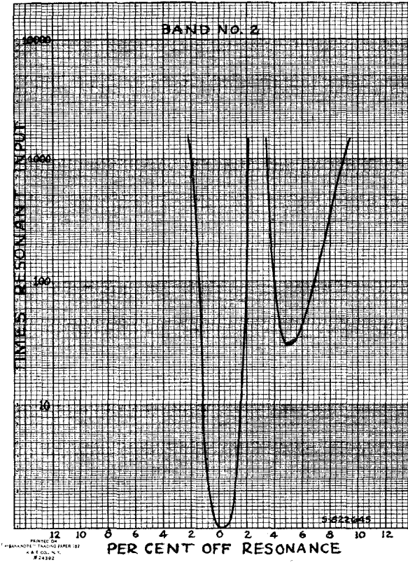
Figure 10—Average Selectivity Curve—CW Interference—Bands 1, 2 and 3
