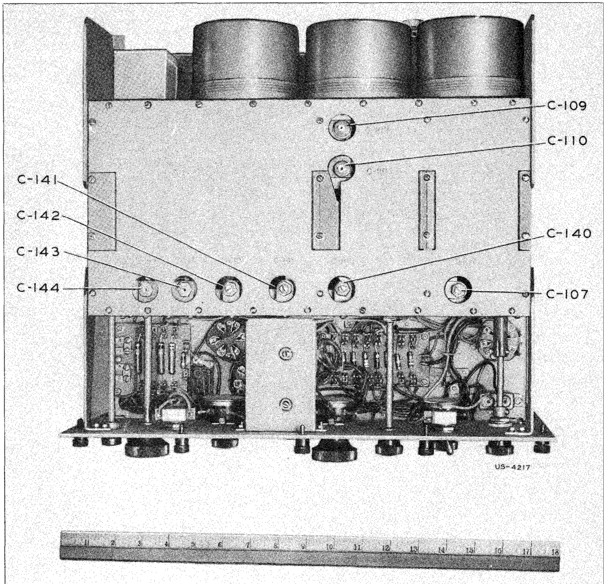
Figure 13—Receiver Unit CRV-46155 (Bottom View of Chassis)
