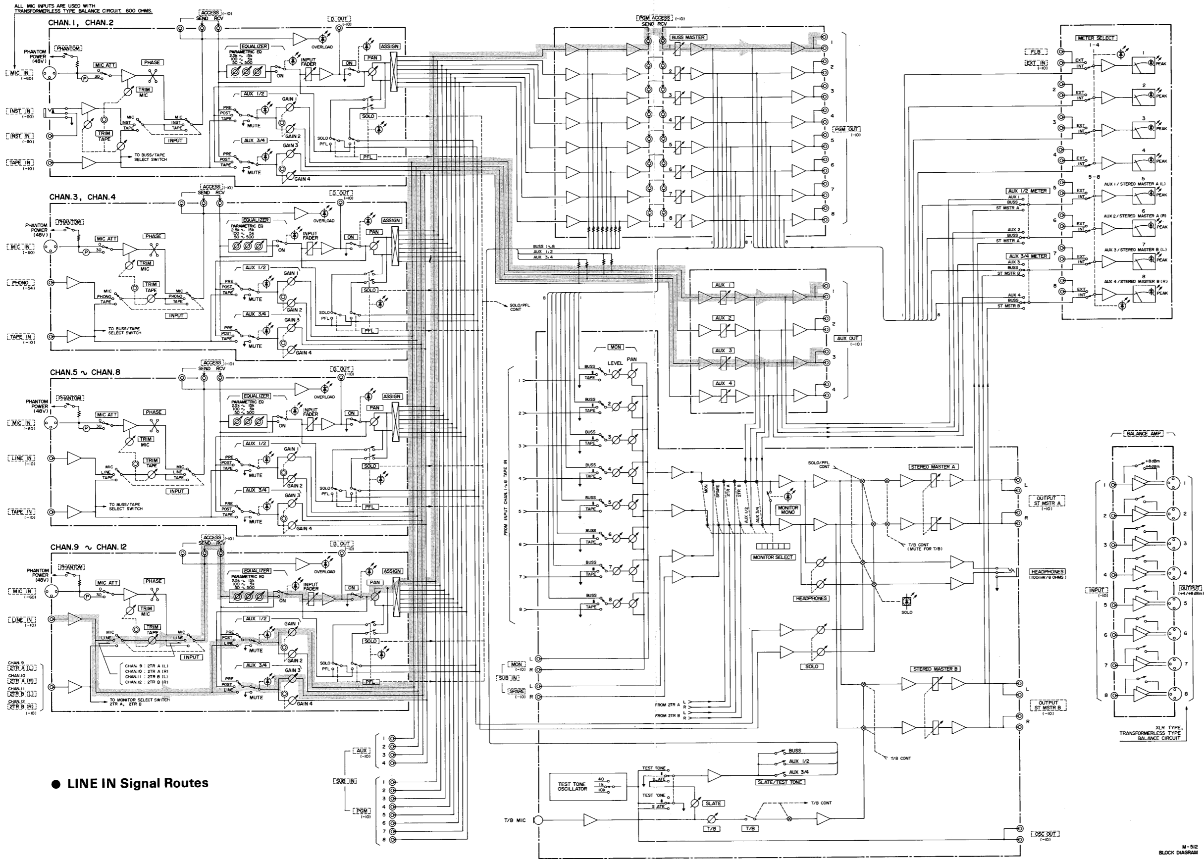
M-512 BLOCK DIAGRAM
