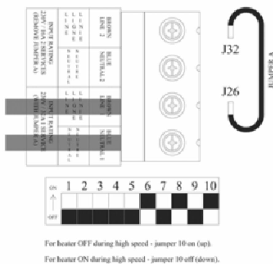
2 16A lines of service. (Remove jumper A)
