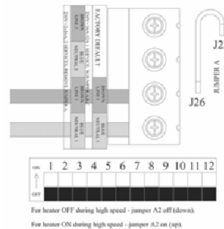
2 16A lines of service (Remove jumper A)
