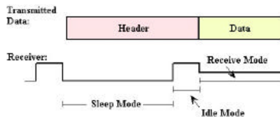
Figure 7b – The length of the long header exceeds the period of Cyclic Sleep. The receiver is guaranteed to detect and receive the data packet.
