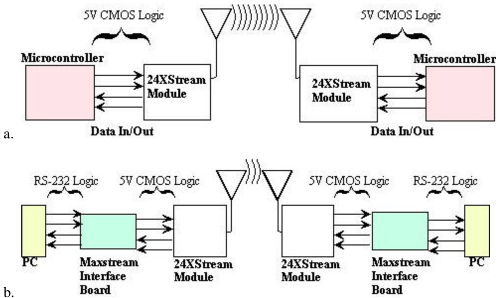
Figure 3 – Diagram of data flow from a microcontroller or PC (or any RS-232 device) through a pair of 24XStream wireless modules to receiving microcontroller or PC. (Note: When connecting the 24XStream to an RS-232 device, the MaxStream Interface Board adjusts voltage levels between the RS-232 device and the MaxStream wireless module.)
