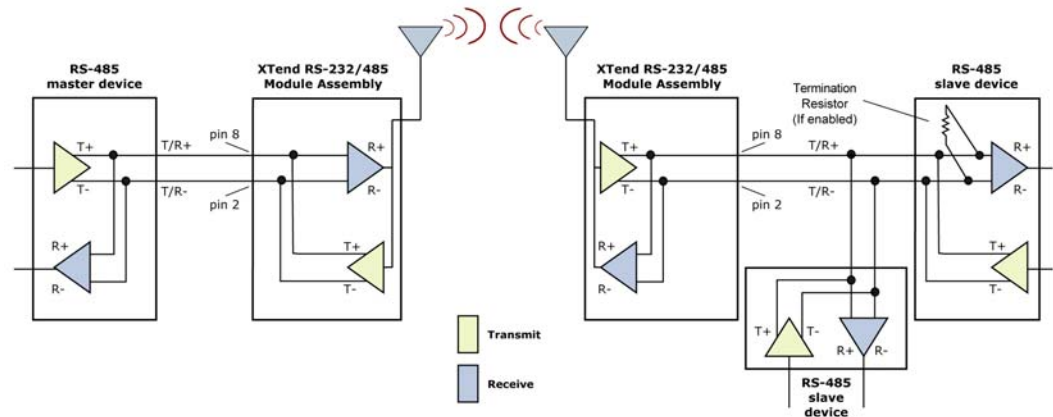
Figure B-19. XTend Module Assembly in an RS-485 (2-wire) half-duplex environment
