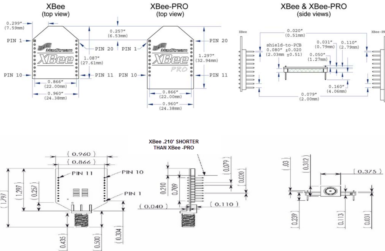
Figure 1-01. Mechanical drawings of the XBee®/XBee-PRO® RF Modules (antenna options not shown) The XBee and XBee-PRO RF Modules are pin-for-pin compatible
