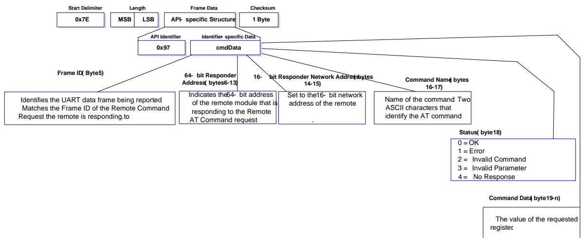
Figure 3-19. Remote AT Command Response.
